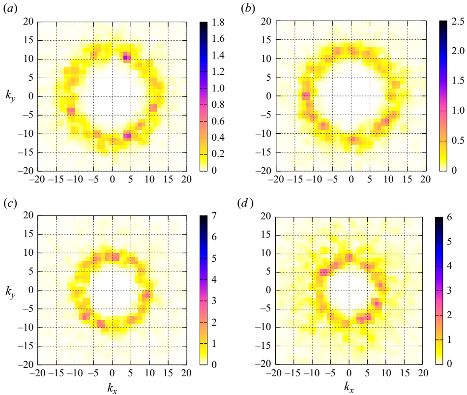
Figure 1. Surfaces of |a_k|^2 \times 10^8 in the condensate region for four simulations of Korotkevich (2023) corresponding to four different mean wave slopes \mu , for (a) \mu = 0.054 , (b) \mu = 0.067 , (c) \mu = 0.093 , (d) \mu = 0.135 .
