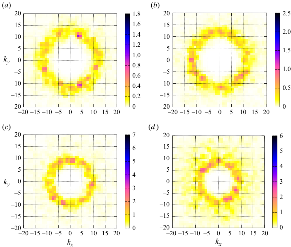
Figure 1. Surfaces of |ak|^2 \times 10^8 in the condensate region for four simulations of Korotkevich (2023) corresponding to four different mean wave slopes \mu , for (a) \mu = 0.054 , (b) \mu = 0.067 , (c) \mu = 0.093 , (d) \mu = 0.135 .
