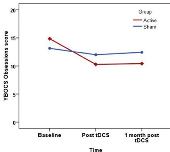
Fig. 1: Mean YBOCS obsessions score in active and sham group over time (N=14)
