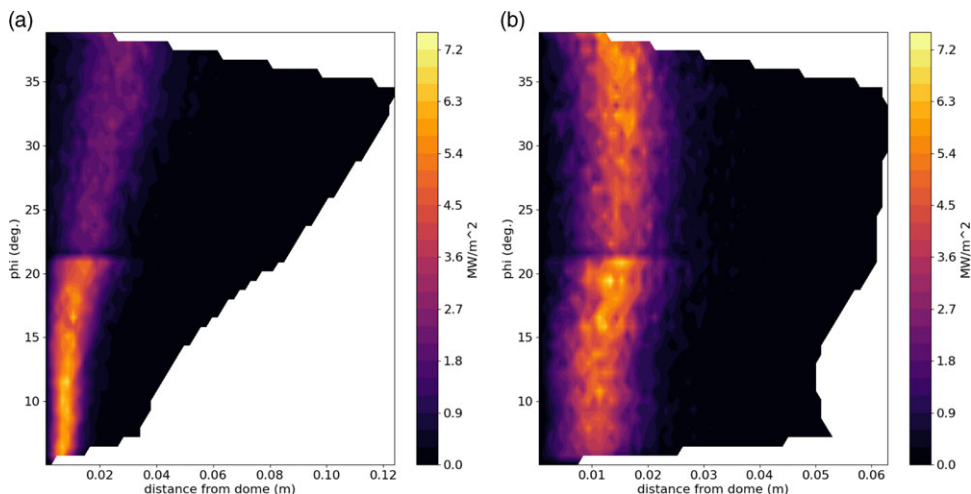
FIGURE 19. Heat flux on the two impact surfaces for d = 1.0 \times 10^{-7} \text{ m}^2 \text{ m}^{-1} .
