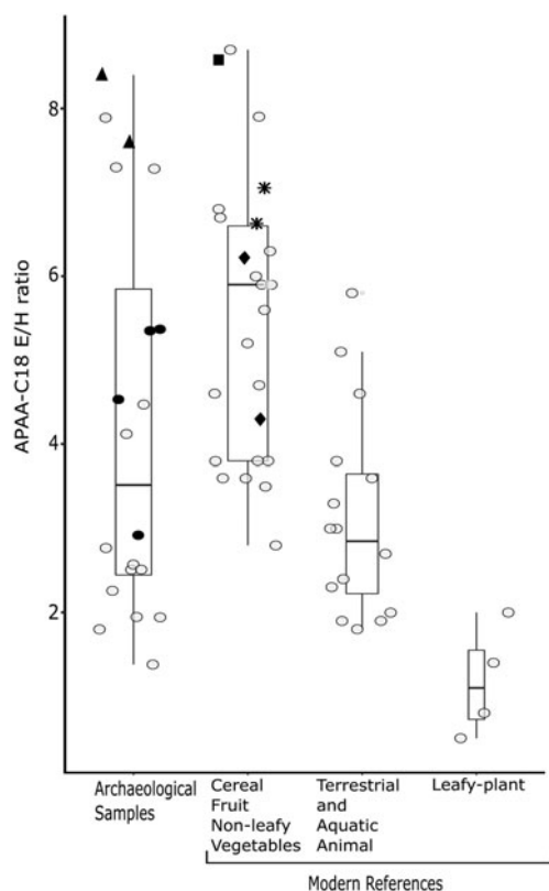
Figure 2. Boxplots of the APAA-C18 E/H ratio of Mocha Island samples. Black circles represent samples with a full set of aquatic biomarkers. The black triangles are samples showing ^{13}\text{C} enrichment of their residues consistent with a \text{C}_4 origin. Black square, asterisks, and diamonds correspond to modern references for Chilean hazelnut, maize, and quinoa, respectively. References are based on Bondetti and others (2020) and this study (see Supplemental Table 5).
