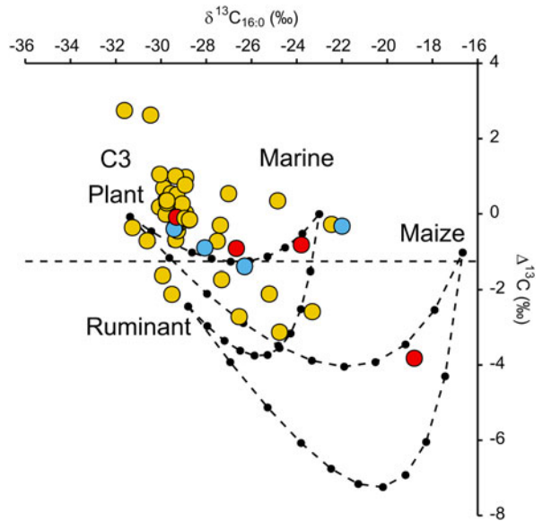
Figure 4. Compound-specific \delta^{13}\text{C} analysis of Mocha Island samples plotted according to their \delta^{13}\text{C}_{16:0} value against \Delta^{13}\text{C}_{\text{C18:0}-\text{C16:0}} . Blue circles indicate the four samples with a full set of aquatic biomarkers. The red circles highlight the samples with an APAA- \text{C}_{18} E/H ratio associated with cereals, fruits, and non-leafy vegetables (Bondetti et al. 2020). Average \delta^{13}\text{C} endpoints were built using modern and archaeological references from published data and this study (see Supplemental Tables 6 and 7). Mixing lines with 10% increments connecting the endpoints were calculated based on the mean relative amount of each alkanoic acid present in the products. Data were gathered from the USDA database. The dashed line indicates a -1.26\text{‰} threshold set for the identification of ruminant carcass fat, as in Dolbunova and colleagues (2023). (Color online)
