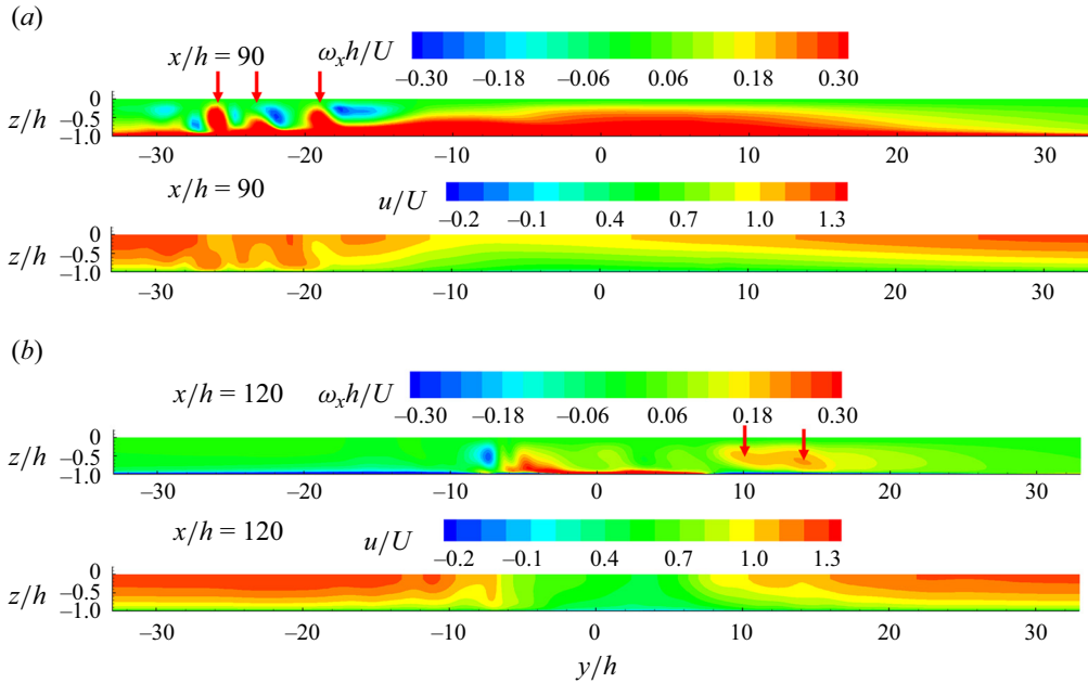
Figure 7. Streamwise vorticity, \omega_x h/U , (top panel) and streamwise velocity, u/U , (bottom panel) in an instantaneous flow field. (a) SVF=1.0, x/h=90 ; (b) SVF=0.1, x/h=120 . The red arrows point towards patches of high streamwise vorticity associated with some of the streamwise-oriented vortices visualized in figure 6.
