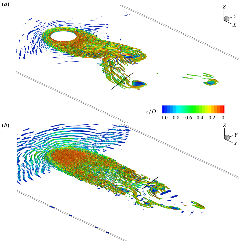
Figure 6. Visualization of coherent structures in the instantaneous flow using a Q isosurface ( Q = 0.002 ). (a) SVF = 1.0 ; (b) SVF = 0.1 . The black lines in panels (a) and (b) show the position of the x/h = \text{constant} planes shown in figure 7.
