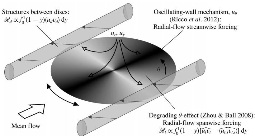
FIGURE 2. Reproduction of figure 14 on p. 557 of Wise & Ricco (2014). Note that the arrows of the interdisc structures now point upstream and upward in the wall-normal direction.
