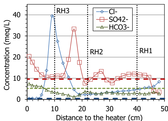
Fig. 11 Main anions measured in aqueous extracts of samples of cell HEE-B (the horizontal lines indicate the concentrations in the untreated pellets and the vertical dotted lines the positions of the sensors)
