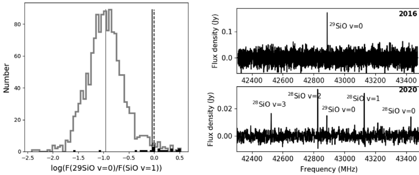
Figure 1. Left: Line ratios between SiO v=1 and ^{29}\text{SiO } v=0 , showing that this ratio is typically around 10:1. Black histogram bins mark where the ^{29}\text{SiO } v=0 line is also detected, demonstrating that the line ratios typical of these detections have much higher ^{29}\text{SiO } v=0 flux than average. Right: Two spectra of the same source taken four years apart demonstrating that 43 GHz isotopologue dominated spectra can drastically change ratios to more typical behavior.
