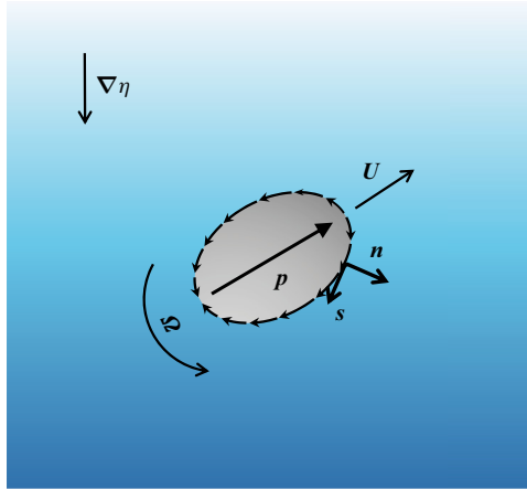
Figure 1. Schematic of a spheroidal swimmer swimming in a constant viscosity gradient \nabla\eta . Here, \mathbf{p} represents the swimming direction of the swimmer.
