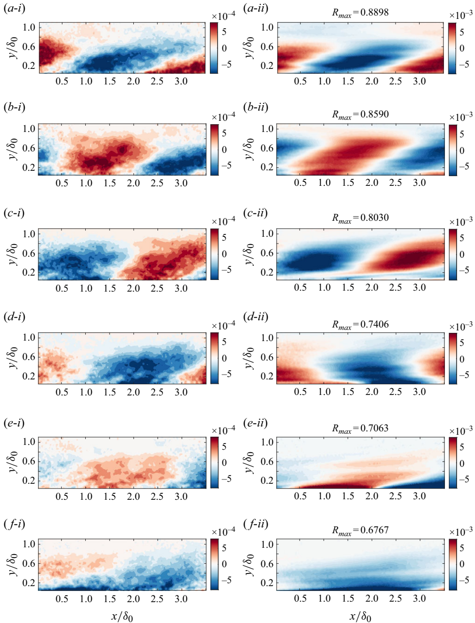
Figure 13. The ST-POD structure considered earlier at six discrete time instances ( i ) and the SPOD structures computed at matched spatial pressure gradient conditions imposed statically ( ii ). The SPOD mode has been chosen to have the same wavelength as the instantaneous ST-POD structure. The phase has been matched using the method described in the text. Here \bar{K} = 0, 0.25, 0.5, 0.74, 0.96 and 1.2 in ( a-f ).
