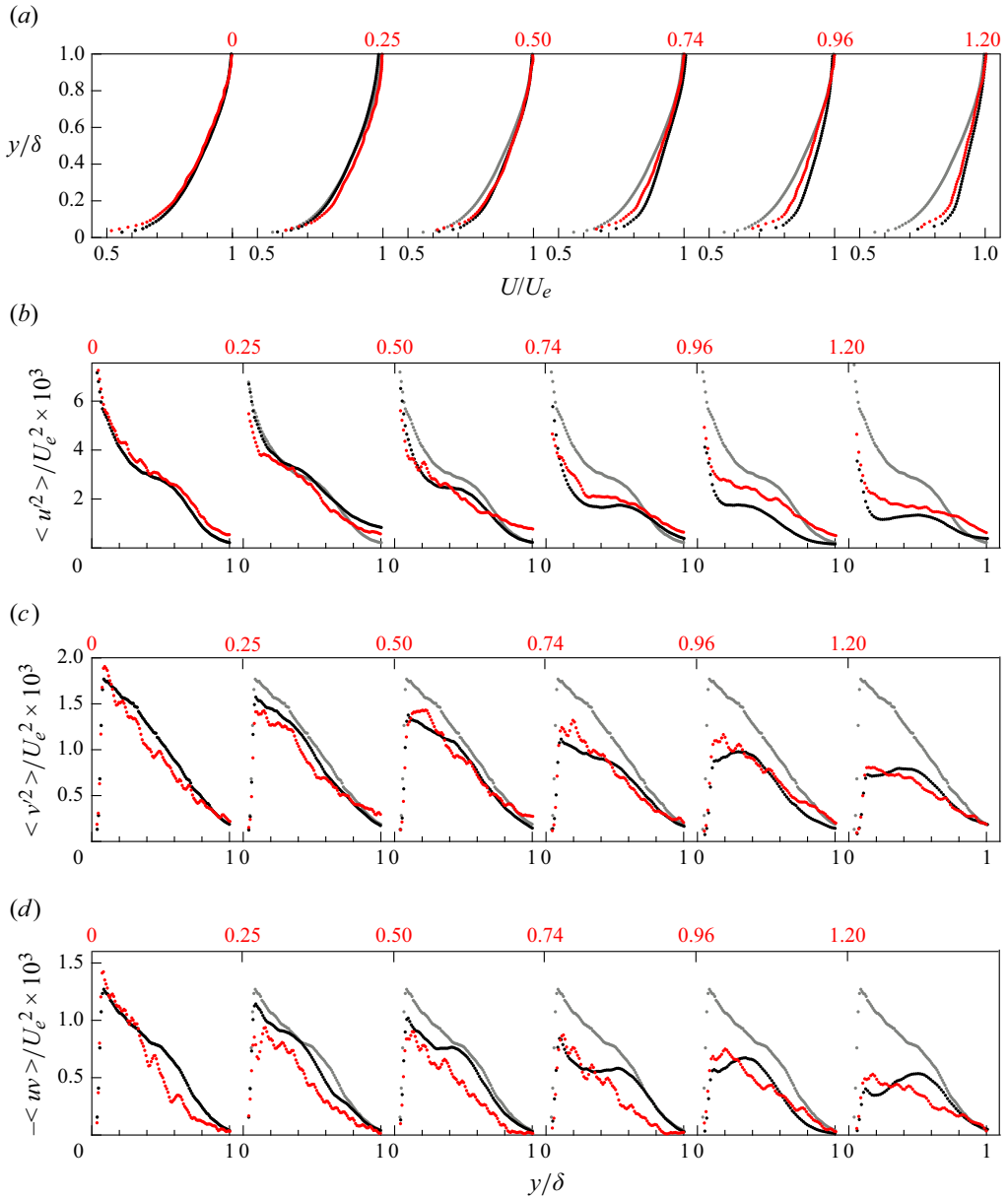
Figure 4. Ensemble-averaged unsteady, outer-scaled turbulent statistics at station A at \bar{K} = 0, 0.25, 0.5, 0.74, 0.96, 1.2 . (a) Mean streamwise velocity profiles. (b) Streamwise Reynolds stress. (c) Wall-normal Reynolds stress. (d) Reynolds shear stress. Profiles at subsequent \bar{K} are shifted by 0.5 units for (a) and 1.1 units for (b), (c) and (d) along the x -axis for visual clarity. Here (---) ZPG, (---) steady FAPG, (---) unsteady FAPG.
