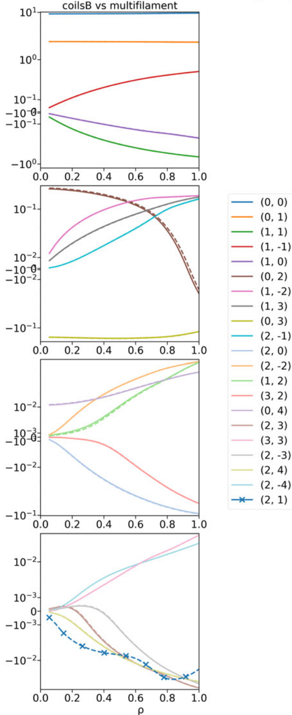
Fourier harmonics of |B| in Boozer coordinates [Tesla]
