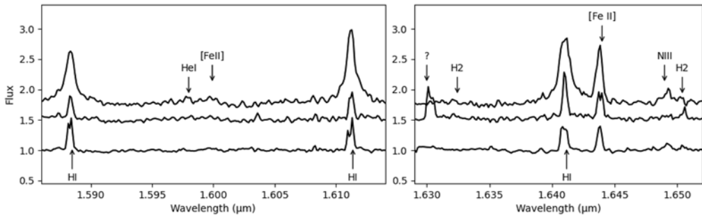
Figure 2. Selected portions of EMIR/GTC H-band spectra of A-SMASHeR targets. Although not being shown here, the K band is also observed by EMIR/GTC.
