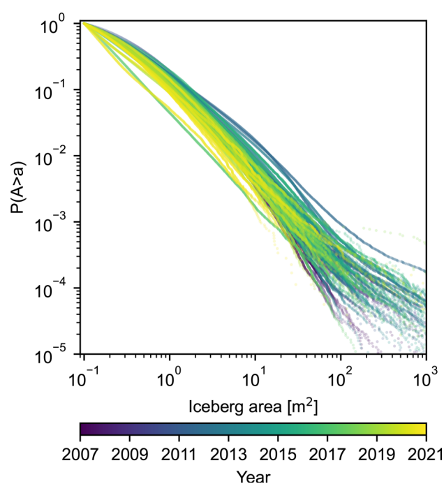
Figure 8. Empirical complementary cumulative distribution function across all aerial surveys.
