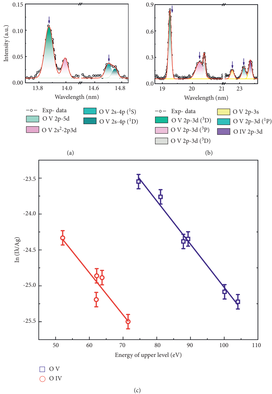
FIGURE 5: Results of plasma temperature. (a, b) The O V characteristic lines (arrows) that were used to construct the Boltzmann plot. Intensities were obtained by line fitting procedure with Gaussian line profiles, and the O IV lines can be treated similarly. (c) Boltzmann plots for O IV and O V emission lines.
