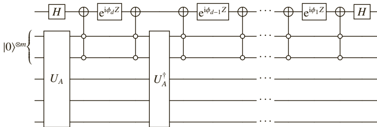
Figure 10.6 The QSVT circuit U_{\Phi} which transforms a block-encoding U_A of A into a block-encoding of f(A) for definite-parity f: [-1, 1] \rightarrow [-1, 1] polynomial of degree d . As discussed in the main text, the angles \{\phi_i\} can be calculated using efficient classical algorithms.
