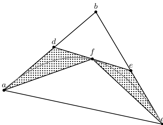
FIGURE 18. Blaschke's property for arcs of parabolas.
