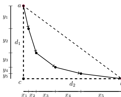
FIGURE 9. A convex chain in a right triangle abc .
