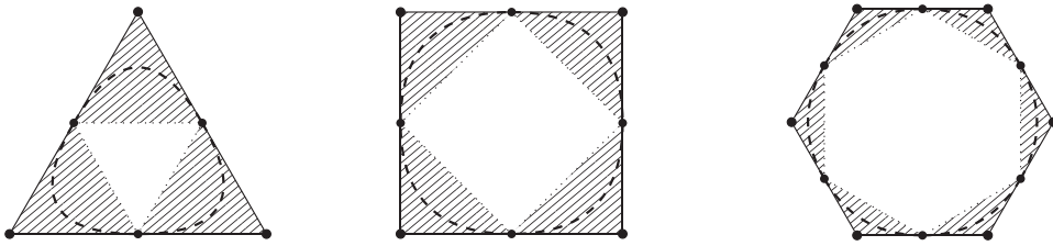
FIGURE 3. For each case \kappa = 3, 4, 6 , the inner dashed curve delimits a convex domain \text{Dom}(\mathfrak{C}_\kappa) inside \mathfrak{C}_\kappa . The dashed curve represents the limit shape of a \mathbf{z}[n] -gon taken under \mathbb{U}_\kappa^{(n)} , conditioned to be in convex position, as n \rightarrow +\infty . The curve can be drawn as follows: add the midpoints of the sides of the initial \kappa -gon, and between two consecutive midpoints, add the arc of the parabola which is tangent to the sides and incident to these inner points. The sum of the hatched areas corresponds to the supremum of affine perimeters (for an explanation see Lemma 17 in the appendix).
