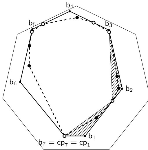
FIGURE 6. In \mathcal{C}_7 , an example of a z[n] -gon, the \text{ECP}(z[n]) , and its vertices b[7] , as well as the first and second corners (the hashed areas). Here we have s[7] = (2, 3, 1, 2, 1, 3, 0) .
