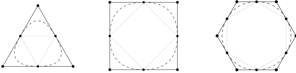
FIGURE 17. For each of the cases \kappa = 3, 4, 6 , the inner dashed curve is the boundary of the domain \text{Dom}(\mathfrak{C}_\kappa) . By the limit shape theorem, it also represents the boundary of a \mathbf{z}[n] -gon where \mathbf{z}[n] is taken under \mathbb{Q}_\kappa^{(n)} , when n \rightarrow +\infty .
