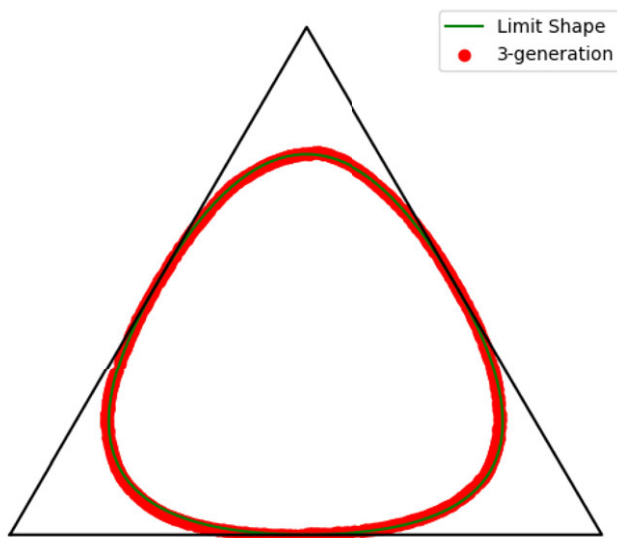
FIGURE 15. A \triangle -sampling, some z[n] -gon for n = 1000 , close to the limit shape.
