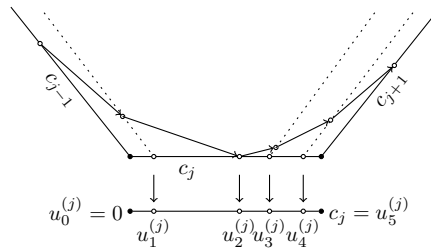
FIGURE 10. The j th side-partition ( 0 = u_0^{(j)} < u_1^{(j)} < \dots < u_{N_j}^{(j)} < u_{N_j+1}^{(j)} = c_j ) of c_j , with s_j = 2 , s_{j+1} = 3 . An alternative way of building the u^{(j)}[N_j, c_j] will be given in Figure 11. Notice here that we see the contact point on c_j , but we do not mark it; we treat it the same as the other points.
