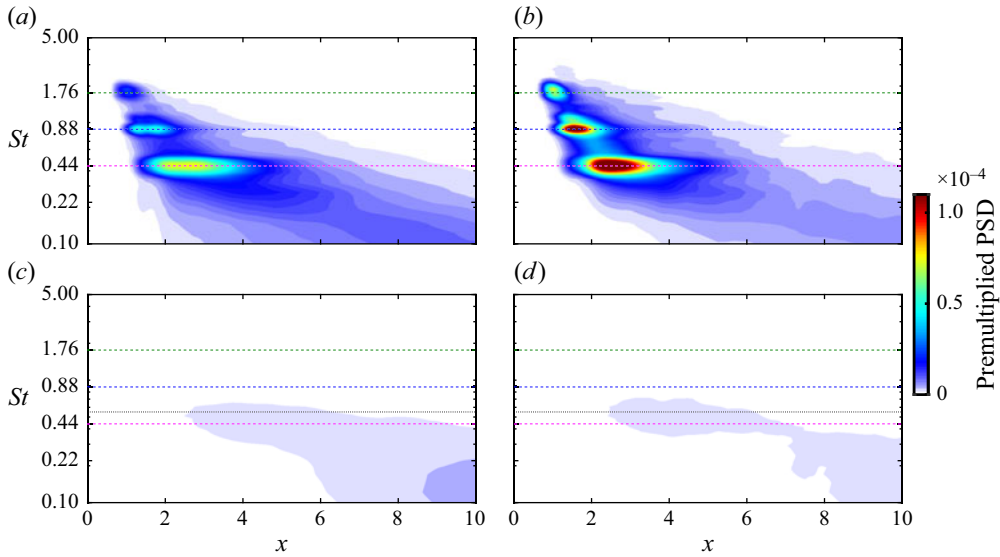
Figure 3. Premultiplied radially integrated PSD, \int_r St \cdot PSDr \, dr , along x for initially laminar jet ( a,b ) and turbulent jet ( c,d ). ( a,c ) Streamwise velocity, u_x ; ( b,d ) radial velocity, u_r . Dashed lines indicate the three tones of the initially laminar jet, and the dotted line corresponds to the most energetic frequency of the turbulent jet.
