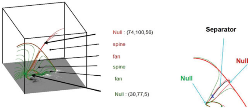
Figure 2. Topological frameworks in AR11158. (Left) All components of the topological framework, 1 unit=1.5 Mm; (Right) Separator connecting nulls in Types A and B
