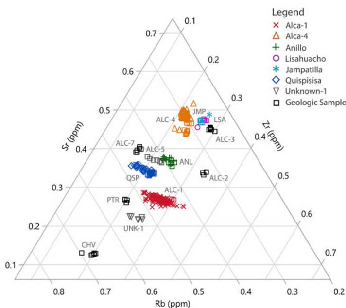
Figure 6. Ternary graph (Sr, Rb, Zr) of obsidian artifacts from the upper Majes-Chuquibamba Drainage by pXRF.
