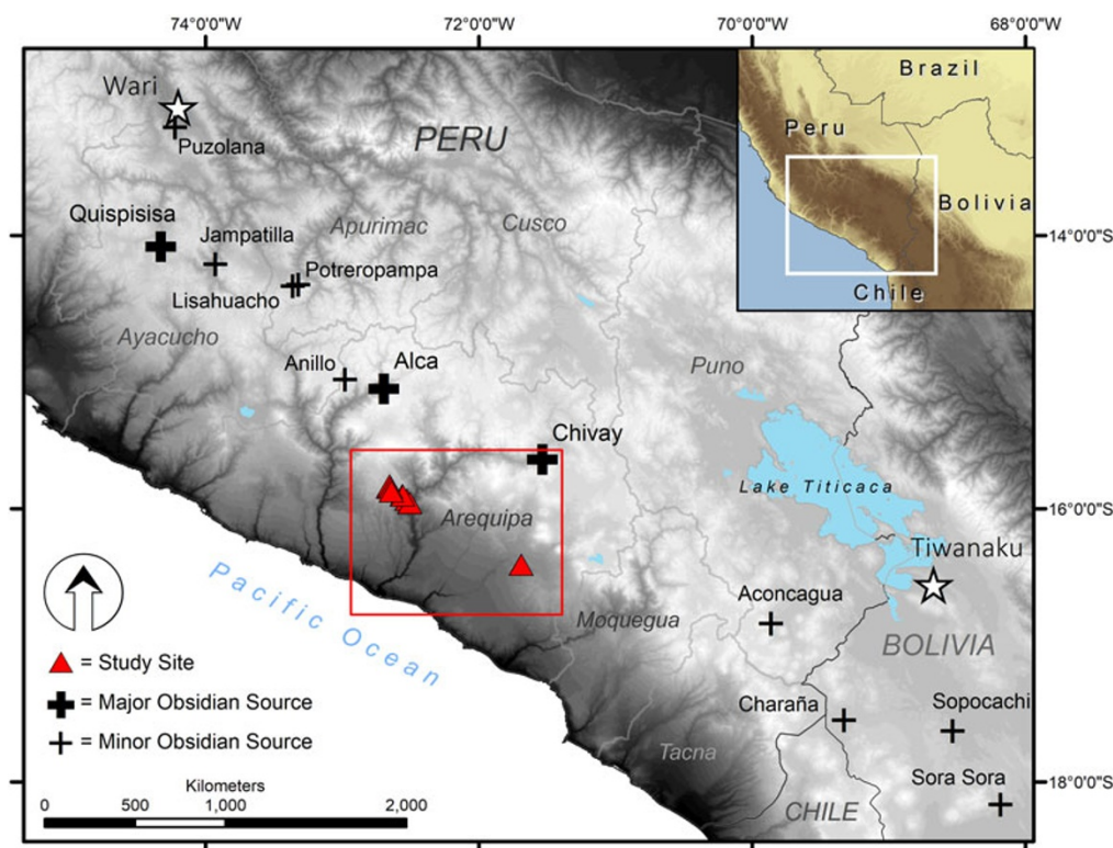
Figure 3. Map of obsidian sources of the south-central Andes in relation to the study region (box) and capitals of the Wari and Tiwanaku states.
