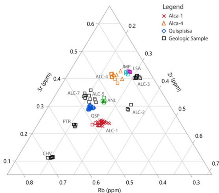
Figure 5. Ternary graph (Sr, Rb, Zr) of obsidian artifacts from Corralones by pXRF.
