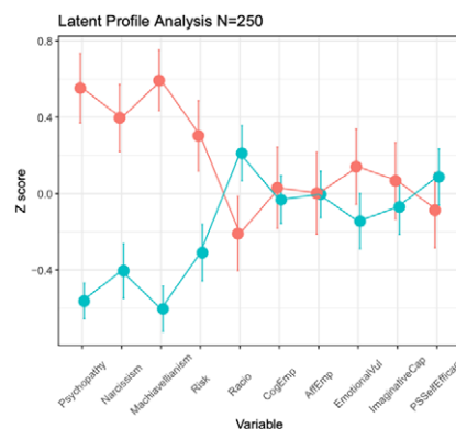
Figure 1. Latent profile analysis
