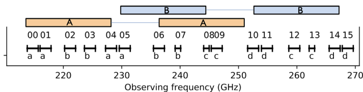
Figure 1. Demonstration of the tuning setup for the ALMA Large Program “ATOMIUM” (2018.1.00659.L, PI: Leen Decin, Decin et al. (2022) ) that observed 17 Oxygen rich evolved stars, including a wide range of maser transitions. This program employed four spectral tunings (with spectral windows denoted by a, b, c, and d labels) in Band 6 (adapted from Gottlieb et al. (2022) ). After the WSU, a similar spectral range can be covered by only two tunings (denoted by tunings A and B) and include additional spectral lines throughout the band. During the 2x BW era of the WSU, up to 16 GHz of the receiver’s IF bandwidth (assumed to be 14 GHz per sideband for Band 6v2) can be correlated per tuning.
