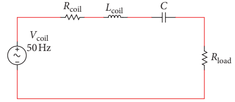
FIGURE 2: The equivalent circuit of the harvesting coil with a matched load.
