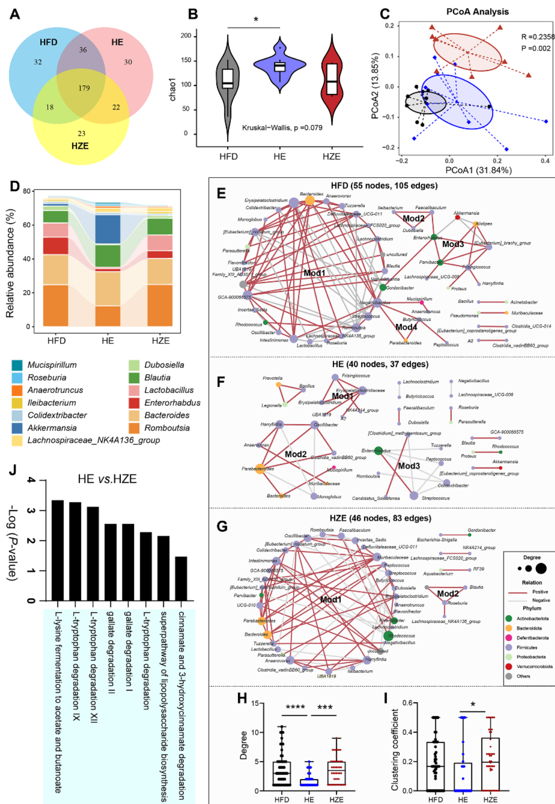
Figure 6. L. reuteri ZJ617 induces alterations in gut microbiome structure and functions. (A) Venn diagram. (B) Chao1 index. (C) Unweighted unifraco PCoA analysis of gut microbiota. (D) Relative abundance. (E-G) Co-occurrence network of HFD, HE and HZE, respectively. (H) Degree. (I) Clustering coefficient. (J) Bar chart represents functional pathways in intestinal contents predicted using PICRUST2.
