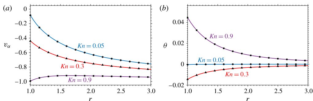
FIGURE 3. The polar velocity v_\alpha at \alpha = \pi/2 and temperature \theta at \alpha = 0 for flow around a sphere. The R13-MFS predictions (●, ▲, ■) for Kn = 0.05, 0.3, 0.9 respectively compared with the analytic result from Torrilhon (2010) (solid lines).
