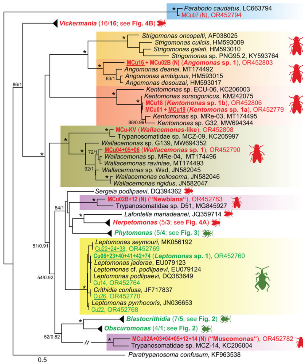
Figure 1. An 18S rRNA-based maximum likelihood phylogenetic reconstruction; sequences from Cuban heteropteran bugs (Cu) are indicated by green, from Cuban dipteran flies (MCu) by red, new species (mOTUs, molecular operational taxonomic units) by bold; isolates with culture established are underlined, (N) indicates detection only by Nanopore sequencing; for details of 5 selected genera see the individual subtrees (Figs 2–4, the number in brackets indicates the number of detected/number of new (in bold) mOTUs); asterisks mark branches with maximal statistical support (ML > 95, Bayesian > 0.95); double crossed branch is 50% of the original length; the scale bar denotes the number of substitutions per site.
