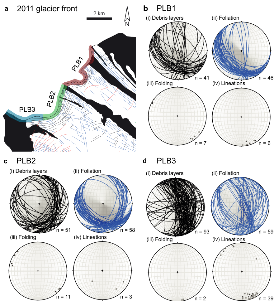
Fig. 7. Three-dimensional data of glaciological structures exposed in the Paulabreen tidewater front. Data are plotted on lower-hemisphere equal-area stereographic projections. Planes (debris layers and foliation) are plotted as great circles. Fold axes and mineral stretching lineations are plotted as points. Legend for structures in (a) is the same as Figure 3.
