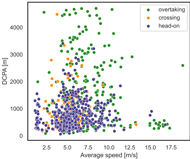
Figure 9. DCPA versus own ship’s average speed during the encounter, according to situation type.
