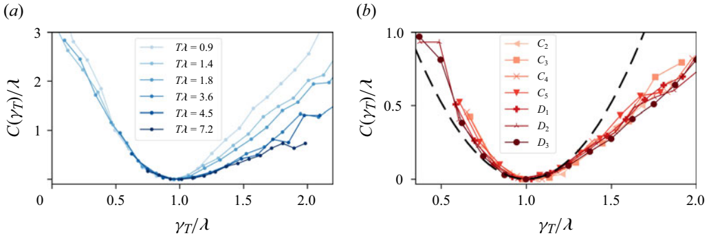
Figure 9. (a) Cramér function for run C_4 and different times. (b) Cramér function for different Re at fixed T\lambda = 7 . The dashed line represents the quadratic form (x - 1)^2/(2\Omega/\lambda) with \Omega/\lambda = 0.24 .
