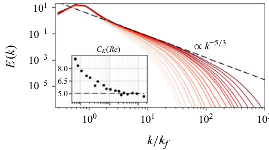
Figure 3. Time-averaged spectra E(k) for all simulations. Colour coding is the same as that of figure 2. Inset: C_K as a function of the Reynolds number.
