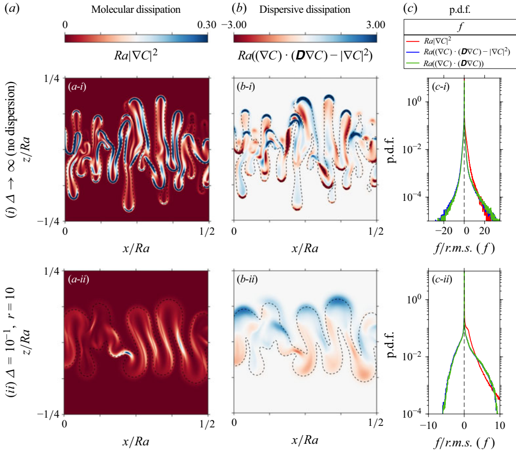
Figure 9. The distributions of (a) molecular ( Ra|\nabla C|^2 , see (3.10)) and (b) dispersive ( Ra[(\nabla C) \cdot (D\nabla C) - |\nabla C|^2] ) scalar dissipation taken at time t = 10^4 . The case without dispersion is shown in (i) ( Ra = 10^4 , \Delta \rightarrow \infty ) and the case with dispersion in (ii) ( Ra = 10^4 , \Delta = 10^{-1} , r = 10 ). For better visualisation, only a small region in the core of the domain is shown ( 0 \leq x/Ra \leq 1/2 , -1/4 \leq z/Ra \leq 1/4 ). The dashed lines represent the iso-contours C = 1/4 and C = 3/4 . (c) The probability density function (p.d.f.) of the components of the molecular, dispersive and total dissipation normalised by their respective root mean squares (r.m.s.) and relative to the specific fields considered. For better visualisation the limits of the colourbars in (a,b) are reduced compared with the maximum/minimum values present in the field.
