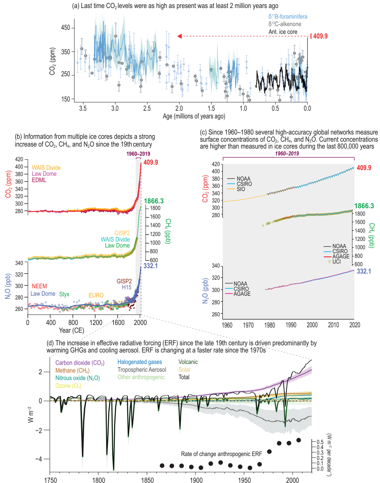
Figure TS.9 | Changes in well-mixed greenhouse gas (WMGHG) concentrations and effective radiative forcing (EFR). The intent of this figure is to show that the changes of the main drivers of climate system over the industrial period are exceptional in a long-term context. (a) Changes in carbon dioxide (CO 2 ) from proxy records over the past 3.5 million years. (b) Changes in all three WMGHGs from ice core records over the Common Era. (c) Directly observed WMGHG changes since the mid-20th century. (d) Evolution of ERF and components since 1750. Further details on data sources and processing are available in the associated FAIR data table. [2.2, Figures 2.3, 2.4 and 2.10]
