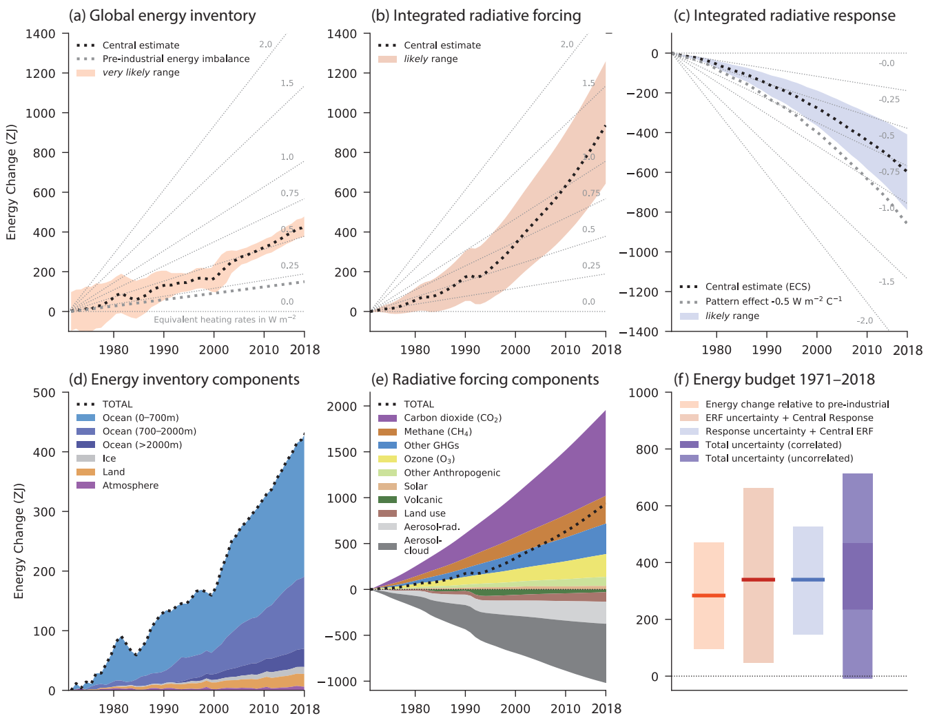
Figure TS.13 | Estimates of the net cumulative energy change ( ZJ = 10^{21} Joules) for the period 1971–2018 associated with (a) observations of changes in the global energy inventory, (b) integrated radiative forcing, and (c) integrated radiative response. The intent is to show assessed changes in energy budget and effective radiative forcings (ERFs). Black dotted lines indicate the central estimate with likely and very likely ranges as indicated in the legend. The grey dotted lines indicate the energy change associated with an estimated 1850–1900 Earth energy imbalance of 0.2 \text{ W m}^{-2} (panel a) and an illustration of an assumed pattern effect of -0.5 \text{ W m}^{-2} \text{ }^{\circ}\text{C}^{-1} (panel c). Background grey lines indicate equivalent heating rates in \text{W m}^{-2} per unit area of Earth's surface. Panels (d) and (e) show the breakdown of components, as indicated in the legend, for the global energy inventory and integrated radiative forcing, respectively. Panel (f) shows the global energy budget assessed for the period 1971–2018, that is, the consistency between the change in the global energy inventory relative to 1850–1900 and the implied energy change from integrated radiative forcing plus integrated radiative response under a number of different assumptions, as indicated in the figure legend, including assumptions of correlated and uncorrelated uncertainties in forcing plus response. Shading represents the very likely range for observed energy change relative to 1850–1900 and likely range for all other quantities. Forcing and response time series are expressed relative to a baseline period of 1850–1900. [Box 7.2, Figure 1]
