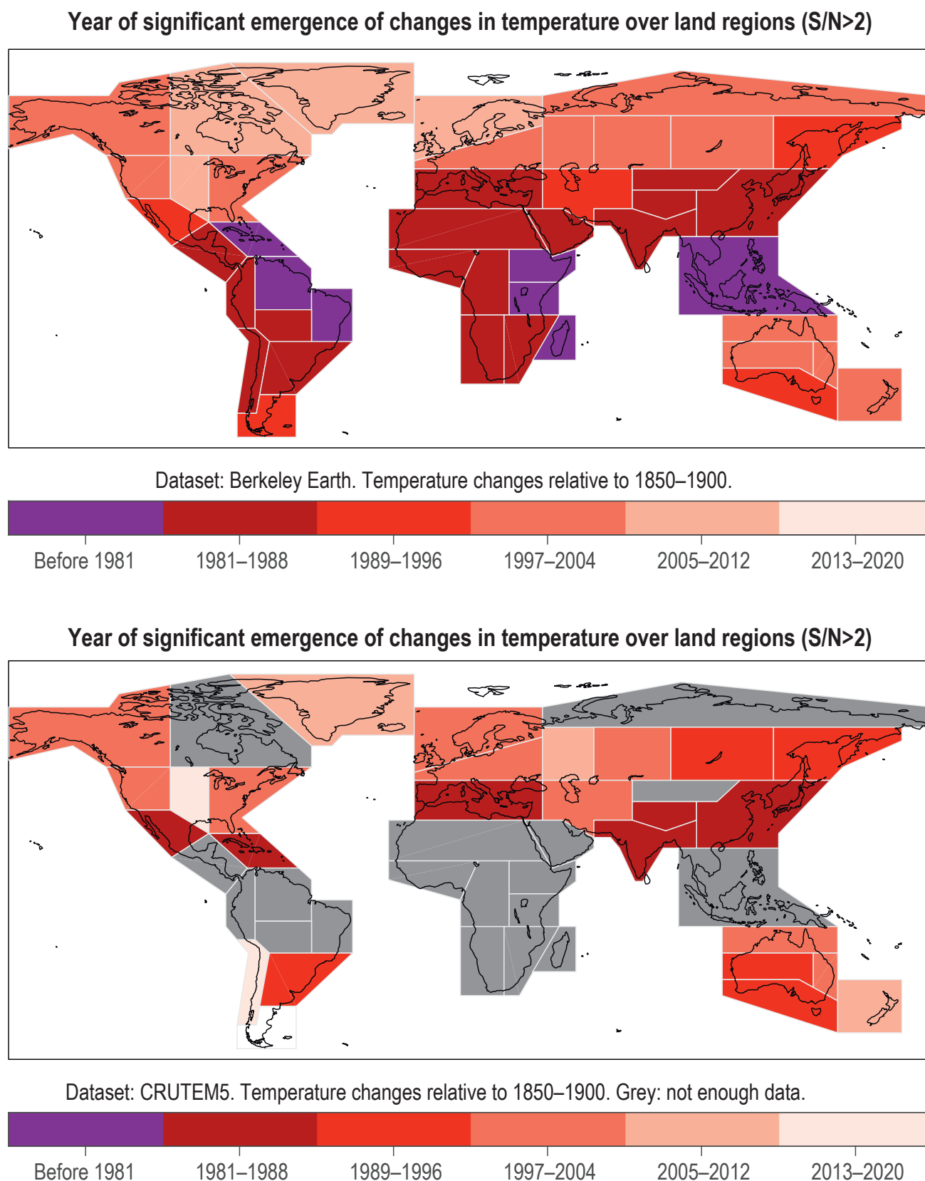
Figure TS.23 | Time period during which the signals of temperature change in observed data aggregated over the reference regions emerged from the noise of annual variability in the respective aggregated data, using a signal-to-noise ratio of two as the threshold for emergence. The intent of this figure is to show, for the AR6 WGI reference regions, when a signal of annual mean surface temperature change emerged from the noise of annual variability in two global datasets and thus also provide some information on observational uncertainty. Emergence time is calculated for two global observational datasets: (a) Berkeley Earth and (b) CRUTEM5. Regions in the CRUTEM5 map are shaded grey when data are available over less than 50% of the area of the region. (Section TS.1.2.4) [Figure Atlas.11]
