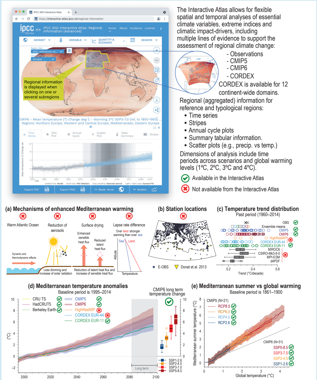
Box TS.12, Figure 1 | Example of generating regional climate information from multiple lines of evidence for the case of Mediterranean summer warming.
