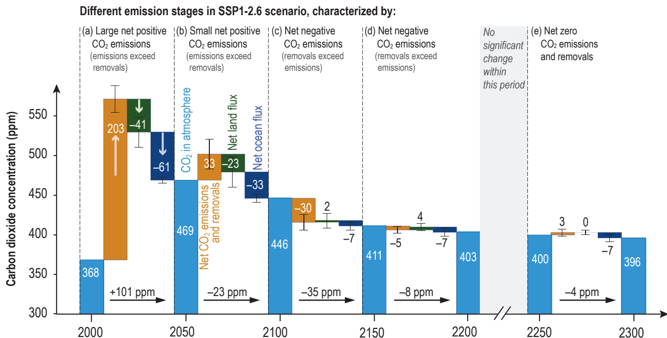
Figure TS.19 | Carbon sink response in a scenario with net carbon dioxide (CO 2 ) removal from the atmosphere. The intent of this figure is to show how atmospheric CO 2 evolves under negative emissions and its dependence on the negative emissions technologies. It also shows the evolution of the ocean and land sinks. Shown are CO 2 flux components from concentration-driven Earth system model (ESM) simulations during different emissions stages of SSP1–2.6 and its long-term extension. (a) Large net positive CO 2 emissions, (b) small net positive CO 2 emissions, (c–d) net negative CO 2 emissions, and (e) net zero CO 2 emissions. Positive flux components act to raise the atmospheric CO 2 concentration, whereas negative components act to lower the CO 2 concentration. Net CO 2 emissions and land and ocean CO 2 fluxes represent the multi-model mean and standard deviation (error bar) of four ESMs (CanESM5, UKESM1, CESM2-WACCM, IPSL-CM6a-LR) and one Earth system model of intermediate complexity (Uvic ESCM). Net CO 2 emissions are calculated from concentration-driven ESM simulations as the residual from the rate of increase in atmospheric CO 2 and land and ocean CO 2 fluxes. Fluxes are accumulated over each 50-year period and converted to concentration units (parts per million, or ppm). {5.6.2.1, Figure 5.33}
