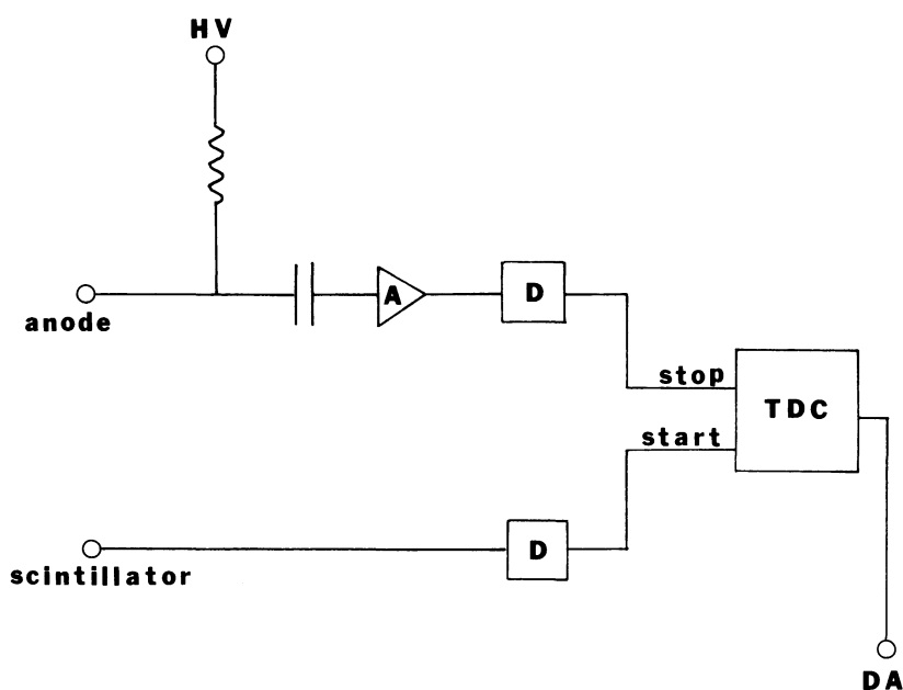
Figure 10.9 Simple readout system for drift chamber signals. (HV) high voltage, (A) preamplifier, (D) discriminator, (TDC) time to digital convertor, and (DA) data acquisition.
