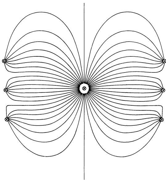
Figure 10.6 Electric field lines in the TASSO drift cell (H. Boerner et al., Nuc. Instr. Meth. 176: 151, 1980.)
