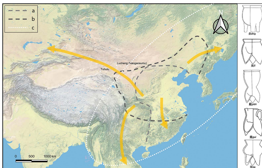
Figure 4. Estimated distributions of tripod pottery vessels li 鬲, ding 鼎, yan 甗, gui 鬺 (or he 盬) and jia 𩰫 before (a) and after 2000 BC (b) and their westernmost appearance in archaeology at Tuhulu and Lucheng, in relation to the distribution of sticky landrace varieties of modern broomcorn millet (c). Arrows indicate millet dispersal routes after Liu et al. (2019) (figure by authors).
