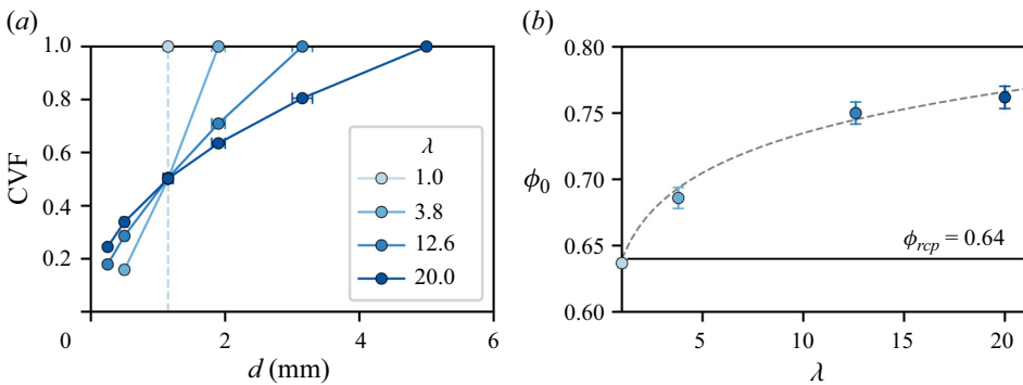
Figure 2. (a) The CVF as a function of the grain diameter d with a distribution following \text{CVF} = (d/d_{\max})^n with n = [1, 1.38, 0.69, 0.47] for the size ratios \lambda = [1, 3.8, 12.6, 20] , respectively. All GSDs have common CVF 0.5 for d_{50} = 1.15 mm. Markers represent the mean size, and horizontal bars represent the ranges in size reported by the supplier. (b) Average sample initial packing fraction \phi_0 as a function of \lambda . The vertical error bars represent the variability among samples with the same polydispersity level. The dashed line follows a power-law function in the form \phi_0 = \lambda^{0.06} \phi_{\text{rcp}} , with \phi_{\text{rcp}} being the random close packing of monodisperse spheres (Scott 1960).
