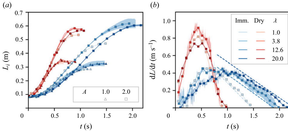
Figure 5. (a) Front position evolution L(t) for dry (red) and immersed (blue) columns, and for A \approx 1 ( \Delta ) and A \approx 2 ( \square ). (b) Front velocity evolution dL/dt for dry and immersed columns with aspect ratio A \approx 2 . Shaded areas represent the variability between repetitions, with envelopes indicating the minimum and maximum values, and markers and continuous lines are the average of them. In (b), the dashed lines represent the collapse acceleration magnitudes d^2L/dt^2 for immersed columns during the collapse deceleration phase.
