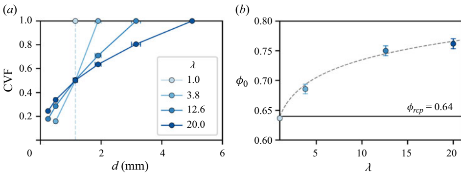
Figure 2. (a) The CVF as a function of the grain diameter d with a distribution following CVF = (d/d_{max})^n with n = [1, 1.38, 0.69, 0.47] for the size ratios \lambda = [1, 3.8, 12.6, 20] , respectively. All GSDs have common CVF 0.5 for d_{50} = 1.15 mm. Markers represent the mean size, and horizontal bars represent the ranges in size reported by the supplier. (b) Average sample initial packing fraction \phi_0 as a function of \lambda . The vertical error bars represent the variability among samples with the same polydispersity level. The dashed line follows a power-law function in the form \phi_0 = \lambda^{0.06} \phi_{rcp} , with \phi_{rcp} being the random close packing of monodisperse spheres (Scott 1960).
