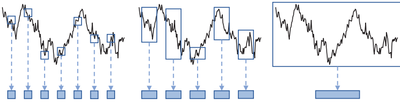
Figure 17 Categorization based on attention modules: point-wise, patch-wise, and series-wise. Examples of models that employ each of those attention types respectively are the Informer, PatchTST, and iTransformer.
