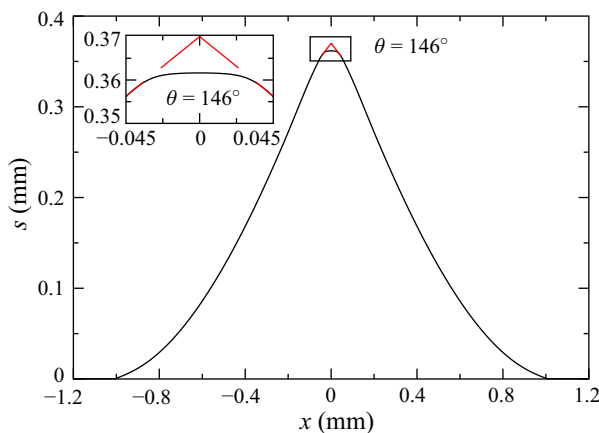
Figure 14. Tip angle near the cusp obtained from our model considering both evaporation and freezing for Ste = 1.22 \times 10^{-3} , T_v = 1 , A_n = 17 , D_g = 2 , D_s = 0.9 , \Lambda_S = 3.89 , \Lambda_W = 698 , \chi = 0.01 , K = 8 \times 10^{-4} , \rho_{veR} = 1 , \Lambda_g = 0.041 , D_w = 15 , RH = 0.70 , \epsilon = 0.2 , D_v = 1.65 \times 10^{-6} , \Delta = 10^{-4} , \Psi = 0.30 and Pe_v = 1 . Note that Marin et al. (2014) experimentally observed a tip angle of \sim 139^\circ .
