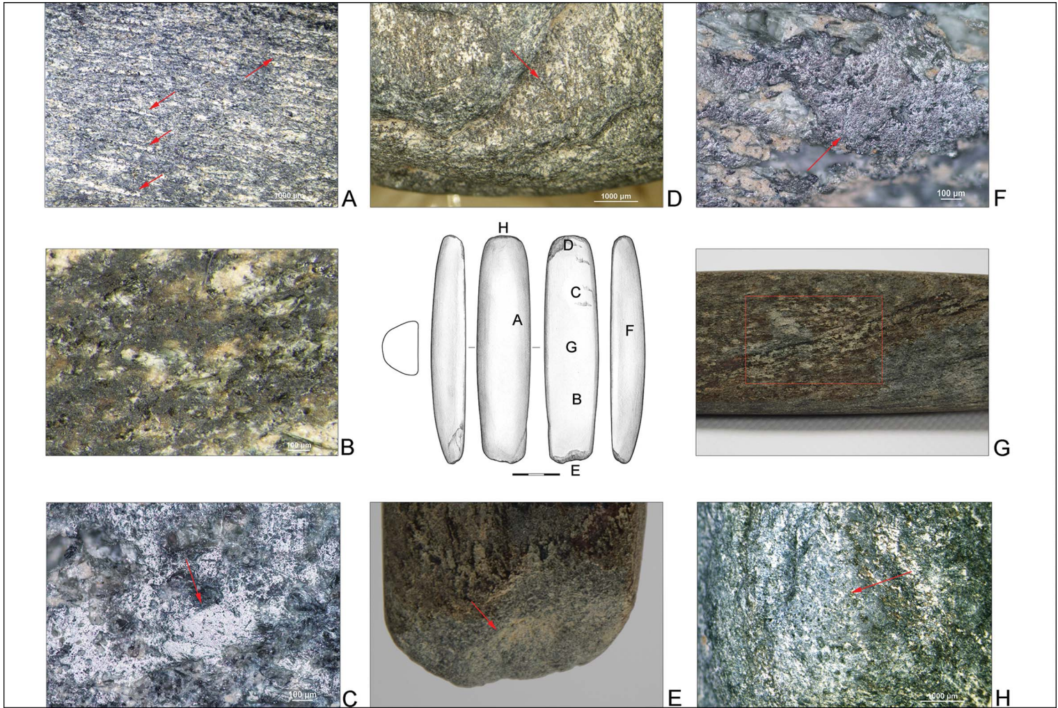
Figure 3. Shoe-last adze from Miłosławice (drawn by N. Lenkow). Traces of production and use (marked with red arrows and box): A) linear grain extractions; B) surface levelling; C) bright polish; D) flaking scars; E) secondary negatives; F) matt polish; G) grain removal on surface; H) butt rounding (photographs by B. Kufel-Diakowska).
