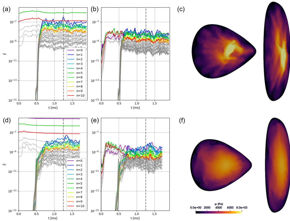
FIGURE 8. Magnetic ( a,d ) and kinetic ( b,e ) energies of W7-AS cases without flows using a Gaussian heating profile ( a–c ) and artificially maintaining the initial equilibrium profiles ( d–f ). The pressure is shown in the \phi = 0 and \phi = \pi poloidal planes ( c ) and ( f ) at the time point corresponding to the grey dashed line. In the case with a Gaussian heat source ( a–c ), the n = 1 magnetic energy is larger than other mode numbers belonging to the N_f > 0 mode families, the energy signature is not sustained, and the case is unstable to multiple, overlapping modes. At t = 1.25 ms, a clear (1, 2) mode structure is present in the pressure ( c ). In the case with a maintained equilibrium profile ( d–f ), a weaker low n magnetic energy signature is observed, which corresponds to the low n perturbation being restricted to the plasma outer midradius.
