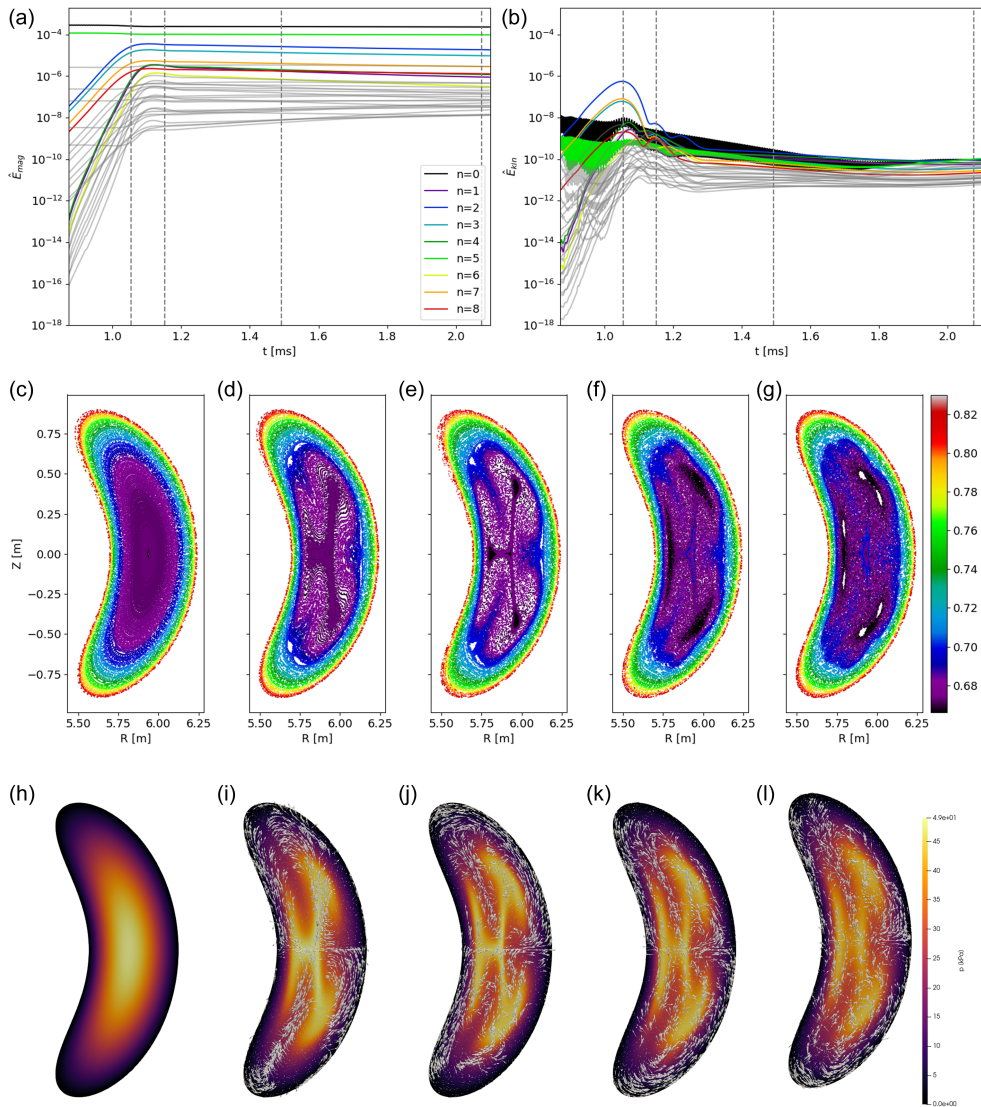
FIGURE 3. Evolution of magnetic ( a ) and kinetic ( b ) energies during the initial nonlinear phase of a (2, 3) interchange mode in a W7-X-like configuration. The initial dynamics of the dominant (2, 3) perturbation is ideal ( c,d ), as illustrated by the nested compression of flux surfaces. Only in the late nonlinear phase ( e–g ), the local \iota value changes due to reconnection of local current sheets. The pressure profile deformation ( h–l ) is approximately aligned with the flux surface deformation.
