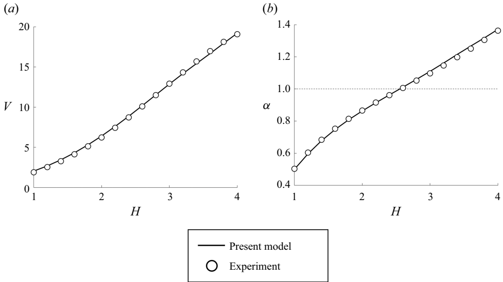
Figure 9. Comparison between experimental and numerical model results under quiescent flow conditions for (a) volume, (b) axis ratio of the drop.
