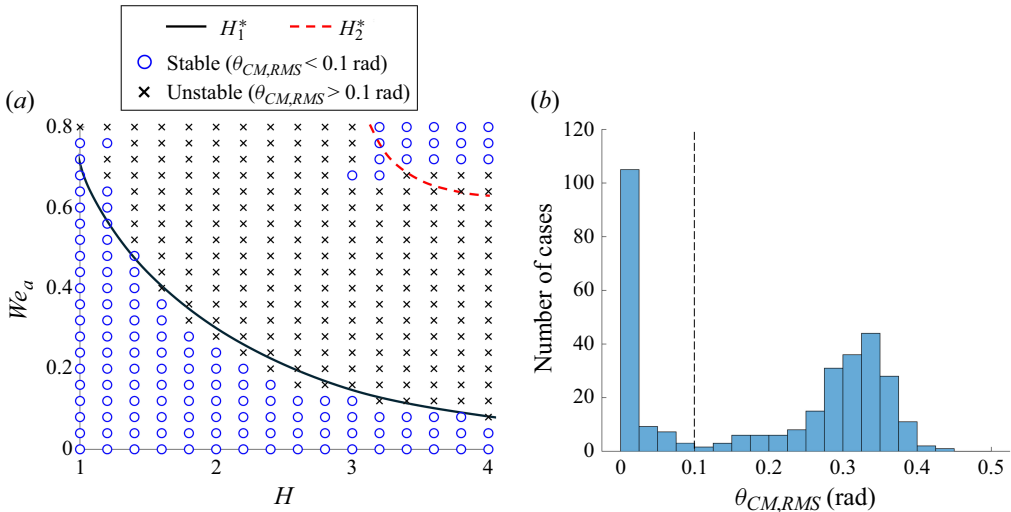
Figure 14. (a) Stability regime map based on experimental data, complemented by predictions from the numerical model. Symbols indicate whether the equilibrium is stable or unstable at specific drop sizes and flow velocities. Curves representing the two critical heights H_1^* and H_2^* , as calculated from the numerical model, are shown with a solid black line and a dashed red line, respectively. (b) A histogram of \theta_{CM,RMS} values from experimental cases, with a dashed line marking the stability threshold.
