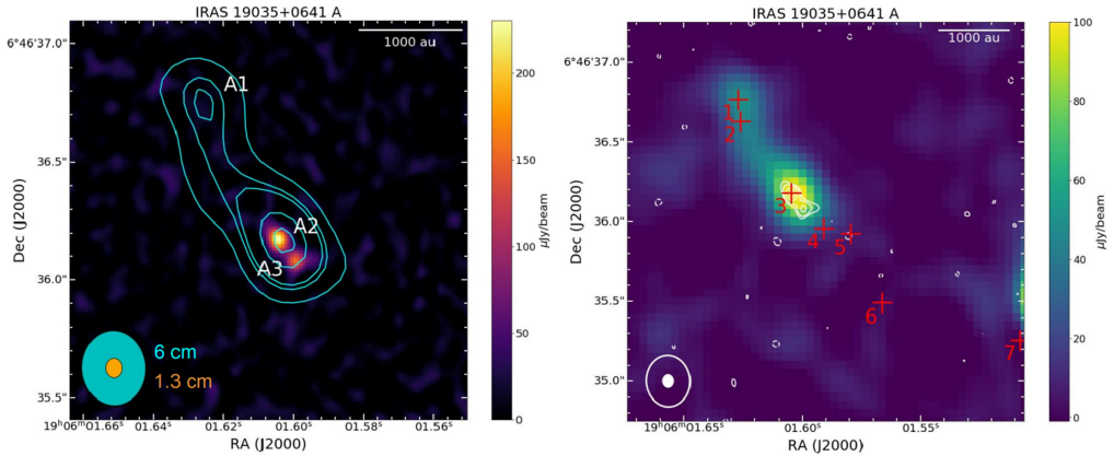
Figure 1. Left: 6 cm (contours, Rosero et al. 2016 ) and 1.3 cm continuum emission (color) toward IRAS 19035+0641 A. The three continuum peaks identified (i.e., A1, A2, A3) are labeled. Right: the 6 and 1.3 cm continuum emission is shown in color and contours (respectively), while the position of the water masers detected in the jet are marked with red + symbols and numbered.
