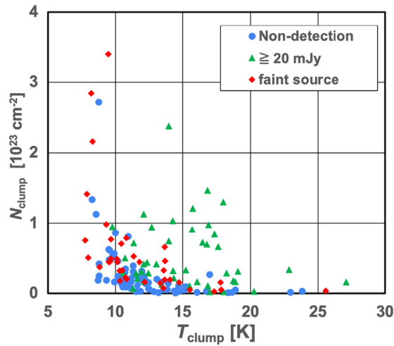
Figure 1. Dust temperatures versus H 2 surface densities for all the targeted clumps. Blue, green, and red markers show non-detection clumps, bright sources, and faint sources ( < 20 mJy), respectively.
