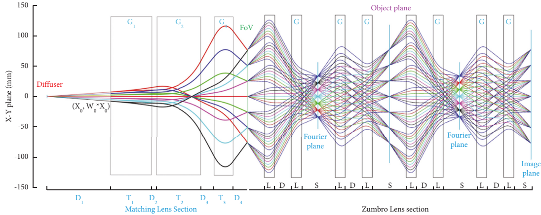
FIGURE 1: Layout of proton beam in radiography system.
