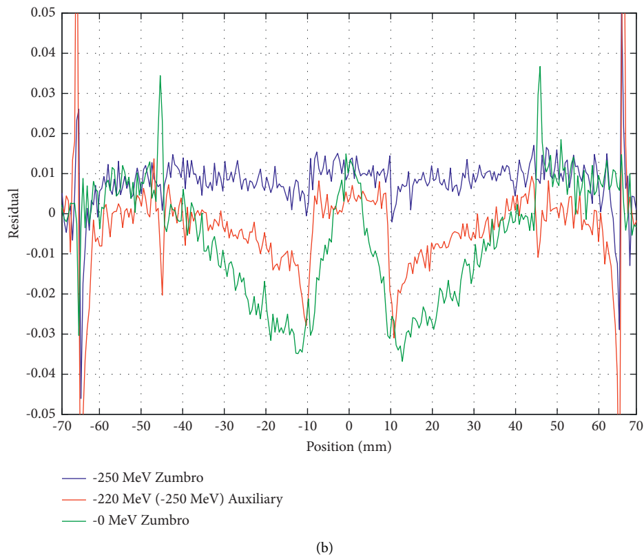
FIGURE 7: Cross-sectional distribution of sphere object. -250\text{ MeV} means the reference momentum is 250\text{ MeV} lower than that of the incident proton ( 20\text{ GeV}/c ). (a) Cross-sectional distribution. (b) Residual error.
