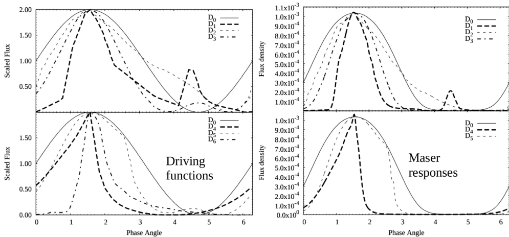
Figure 1. Sample periodic driving functions (left panel) and maser responses (right panel). The driving functions are, D_0 : sinusoid, D_1 : IR continuum digitized from Stecklum et al. (2018), D_2 : theoretical Cepheid light curve from Bhardwaj et al. (2017), D_3 – D_5 : light curves for stars only, shock only, and combined effect by van der Walt et al. (2016) from the spiral shock model of Parfenov and Sobolev (2014), D_6 : background radiation light curve from the colliding wind eccentric binary model by van der Walt et al. (2009). The responses were generated from models with a maser depth range of 5.0–10.0 between quiescent and flare peaks, and for a prolate cloud viewed along its long axis.
