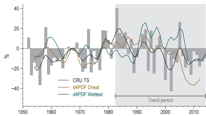
Figure 10.13 | Attribution of the south-western North America precipitation decline during the 1983–2014 period. (a) Water year (October to September) precipitation spatial linear trend (in percent per decade) over North America from 1983 to 2014. Trends are estimated using ordinary least squares. Top row: observed trends from CRU TS, REGEN, GPCC, and the Global Precipitation Climatology Project (GPCP). Middle row: driest, mean and wettest trends (relative to the region enclosed in the black quadrilateral, bottom row) from the 100 members of the MPI-ESM coupled SMILE. Bottom row: driest, mean and wettest trends relative to the above region from the 100 members of the d4PDF atmosphere-only SMILE. (b) Time series of water year precipitation anomalies (%; baseline 1971–2000) over the above south-western North America region for CRU TS (grey bar charts). Black, brown and green lines show low-pass filtered time series for CRU TS, driest and wettest members of the d4PDF SMILE, respectively. The filter is the same as the one used in Figure 10.10. (c) Distribution of south-western region-averaged water-year precipitation 1983–2014 trends (in percent per decade) for observations (CRU TS, REGEN, GPCC and GPCP, black crosses), CMIP6 all-forcing historical simulations (red circles), the MIROC6, CSIRO-Mk3-6-0, MPI-ESM and d4PDF SMILEs (grey box-and-whisker plots). Grey squares refer to ensemble mean trends of their respective SMILE and the red circle refers to the CMIP6 multi-model mean. Box-and-whisker plots follow the methodology used in Figure 10.6. Further details on data sources and processing are available in the chapter data table (Table 10.SM.11).
