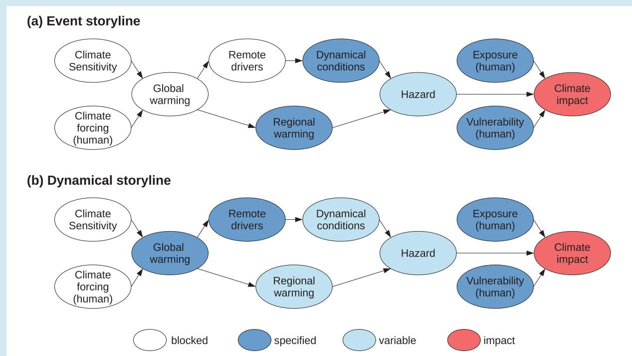
Box 10.2, Figure 1 | Schematic of two types of physical climate storylines with a particular climate impact of concern (red). The storylines are defined by specified elements (dark blue). Variable elements (light blue) are simulated conditional on the specified elements. The white elements are 'blocked' since their state does not need to be known to determine the light blue elements. Other types of storylines could be defined by specifying other elements (e.g., storylines of different climate sensitivities or different representative concentration pathways). (a) Event storyline, where the particular dynamical conditions during the event as well as the regional warming are specified and control the hazard arising from the event. (b) Dynamical storyline, where the global warming level and remote drivers are specified and control the long-term changes in atmospheric dynamics and regional warming. In both storylines, the impact is also conditioned on specified exposure and vulnerability. Figure adapted from Shepherd (2019).
