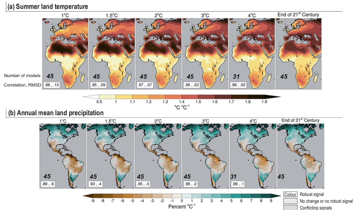
Figure 10.14 | Robustness and scalability of anthropogenic signals at regional scale. (a) Spatial patterns of European and African summer (June to August) surface air temperature change (in ^{\circ}\text{C } ^{\circ}\text{C}^{-1} ) from the Coupled Model Intercomparison Project Phase 6 (CMIP6) multi-model mean (45 models, one member per model, historical simulations and scenario SSP5-8.5) at different global warming levels (GWs) and the end-21st century scaling pattern estimated from the multi-model mean difference between 2081–2100 and the pre-industrial period (1850–1900) divided by the corresponding global mean warming. The scale of all GWL patterns has been adjusted to a global mean warming of 1°C (for example, the resulting 3°C spatial pattern has been divided by three). The scales of the GWL patterns have to be multiplied by their threshold values to obtain the actual simulated warming. The metrics shown in the bottom left corner of the GWL pattern plots indicate the spatial pattern correlation and the root-mean-square difference between the GWL patterns and the scaling pattern. The number in bold just above the metrics gives the number of used CMIP6 models (out of 45) that have reached the GWL threshold. Areas with robust change (at least 66% of the models have a signal-to-noise ratio greater than one and 80% or more of the models agree on the sign of the change) are coloured with no pattern overlaid (Cross-Chapter Box Atlas.1). Areas with a significant change (at least 66% of the models have a signal-to-noise ratio greater than one) and lack of model agreement (meaning that less than 80% of the models agree on the sign of the change) are marked by cross-hatching. Areas with no change or no robust change (less than 66% of the models have a signal-to-noise ratio greater than one) are marked by negatively sloped hatching. (b) Same as (a) but for North, Central and South America annual mean precipitation relative change (percent ^{\circ}\text{C}^{-1} ). The baseline for precipitation climatology is 1850–1900. Further details on data sources and processing are available in the chapter data table (Table 10.SM.11).
