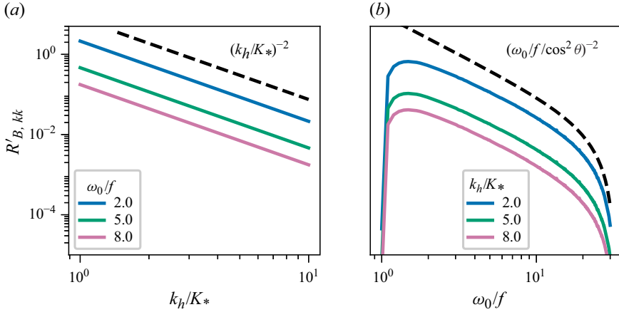
Figure 9. Cross-sections of radial ratio R'_{B,kk} (3.40a), as shown in figure 8, for constant (a) \omega_0/f and (b) k_h/K_* . The (\omega_0/f / \cos^2 \theta)^{-2} prediction of Appendix B.2 is, for small \theta , an (\omega_0/f)^{-2} power law.
