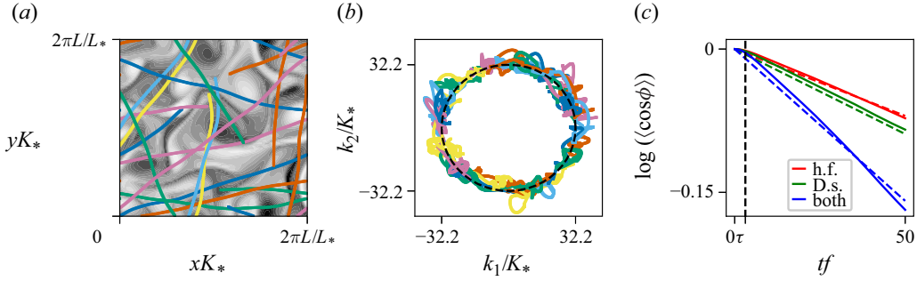
Figure 4. Ray trajectories satisfying the characteristic equations (3.35 a, b ), propagating in the flow described in § 3.2 with Ro = 0.03 , Bu = 0.32 and K_* = 3.10 . (a) A sample of 10 rays in physical space superimposed on the flow vorticity field (darker sections indicate higher-magnitude vorticity). (b) A sample of 50 rays in spectral space initialised on a constant-frequency circle given by the dotted black line. (c) The exact solution (3.32) approximated by the rays' ensemble average (solid lines) and the diffusivity (3.26) (dashed lines). Red lines are calculated solely with the height fluctuation terms in (3.26) and (3.35 a, b ); green lines are solely Doppler shift and; blue lines are the entire system with both Doppler and height fluctuation effects. The vertical dashed line indicates \tau , the point at which the gradient calculation for figure 5 begins.
