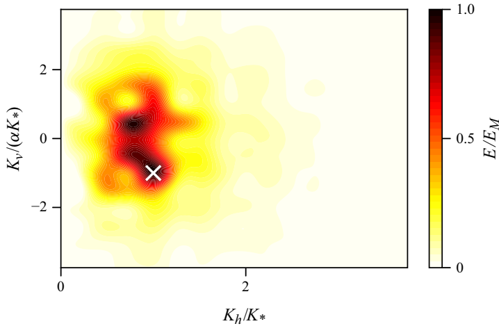
Figure 7. The geostrophic flow component E , smoothed and scaled by a maximum value E_M , of the full Boussinesq simulation in CKV (2023). The horizontal and vertical flow wavenumbers ( K_h, K_v ) are scaled by the characteristic wavevector ( K_h, K_v ) = ( K_*, \alpha K_* ) – with \alpha the aspect ratio of the flow (2.16) – marked by a white cross, at which the geostrophic energy is maximum.
