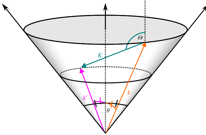
Figure 6. Schematic of the scattering interaction between an incident wave \mathbf{k} and the background flow \mathbf{K} resulting in a scattered wave \mathbf{k}' . The two waves have the same frequency \omega_0(\theta) and thus the background flow connects two points on the constant-frequency cone. For an arbitrary scattering interaction, angle \Theta of the flow's wavevector is bounded between \theta and \pi - \theta , i.e. the angular range of a vector between any two points on the cone.
