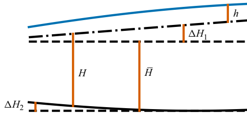
Figure 11. Shallow-water set-up with bottom topography, a modified version of figure 1(b) . The free surface is the solid blue line, the bottom is the solid black line and the horizontal dashed lines enclose the constant mean height \bar{H} . The wave perturbations are given by h and the fluctuation in height due to geostrophy, the dashed-dotted line, is given by \Delta H_1 . The topographic variation in height is \Delta H_2 , which is a negative quantity at the labelled location in this figure.
