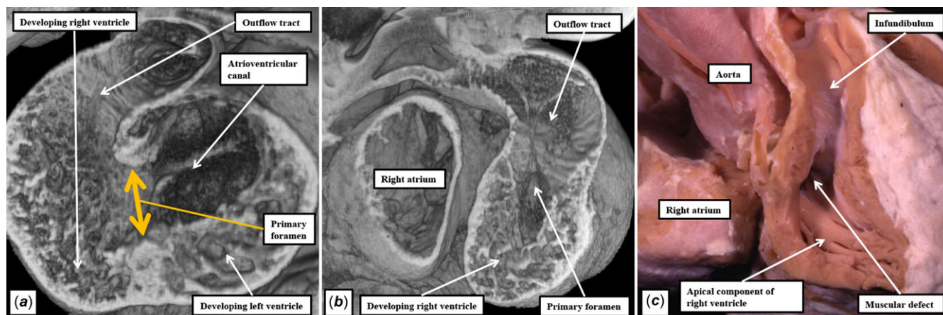
Figure 11. Panels A and B are taken from an epicopic dataset prepared from a mouse embryo sacrificed at embryonic day 10.5. At this stage, the atrioventricular canal is supported exclusively by the developing left ventricle, while the outflow tract arises in its entirety above the cavity of the developing right ventricle. As shown in panel A, all the blood entering the left ventricle must pass through the primary interventricular foramen to reach the developing right ventricle. Panel B shows that the right ventricle has already acquired its apical component. The chamber can be compared to the incomplete right ventricle shown in panel C, which is from an individual with classical tricuspid atresia. The chamber is incomplete because it lacks any direct inlet from the morphologically right atrium.
