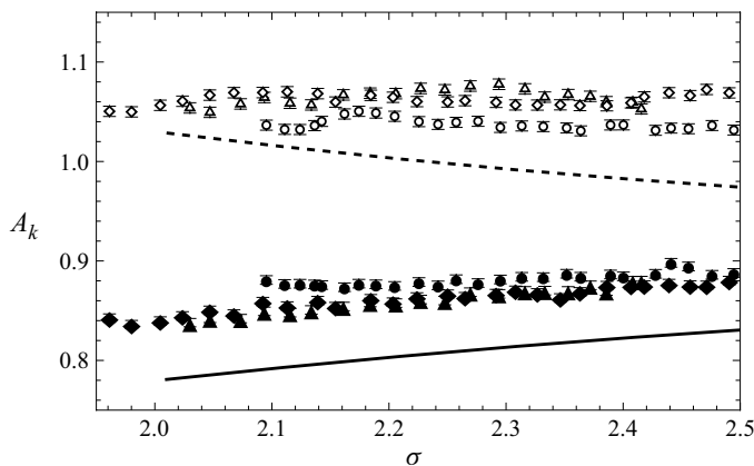
Figure 15. The in-plane bubble aspect ratios, A_k , versus separation, \sigma , for the rear bubble ( k = 1 , dashed curve and open markers) and the front bubble ( k = 2 , solid curve and filled markers), with \delta = 2.86 and \epsilon = 0.027 . The points show experimental measurements and the curves are the asymptotic predictions (6.10). The different marker shapes (triangle, circle, diamond) represent distinct pairs of bubbles that were tracked and measured as the rear bubble caught up and collided with the front bubble. The error between experiment and theory is approximately 6%–10%.
