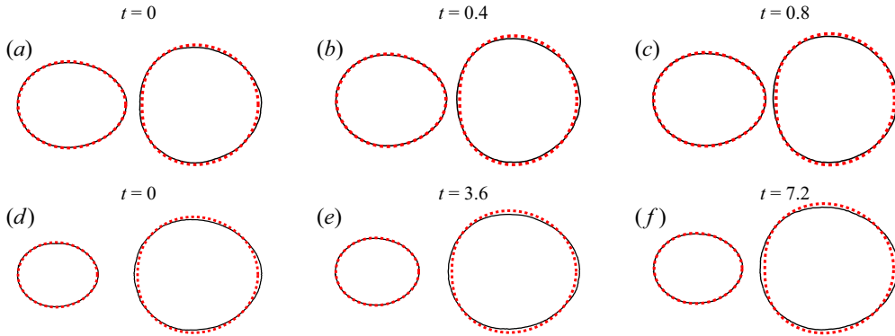
Figure 16. Experimental bubble shapes (black solid), asymptotic solution (6.5) and (6.8) (red dashed) for (a–c) R = 1.23 , \delta = 2.55 and \sigma = (a) 2.39, (b) 2.34, (c) 2.28, (d–f) R = 1.65 , \delta = 1.94 and \sigma = (d) 3.45, (e) 3.23, (f) 2.94. The corresponding different dimensionless times t = \hat{t}\hat{U}/\hat{R}_1 are shown above for the experiments. The background flow is from left to right. Experimental images have been rescaled by the rear bubble radii, \hat{R}_1 = (a–c) 2.9 mm and (d–f) 4.8 mm, for comparison with the theory. The bubble shapes from experiment and asymptotics are aligned so that the centroids of the bubble pairs coincide.
