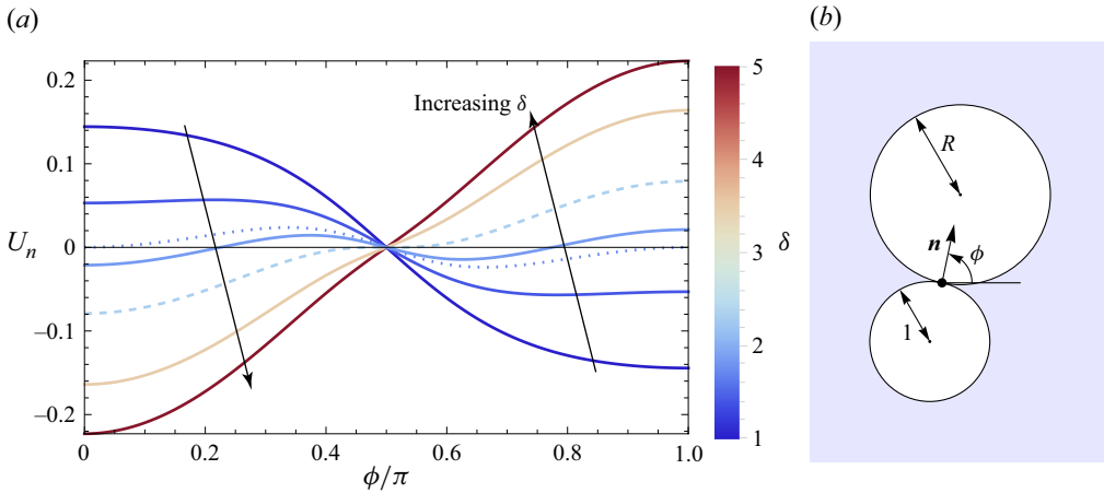
Figure 12. (a) The relative normal velocity, U_n , of the two bubbles as a function of the polar angle, \phi , for a fixed R = 2 and \delta shown by the colour bar. The dotted and dashed curves show U_n as a function of \phi at \delta = \delta_1(2) , and \delta = \delta_2(2) , respectively (see § 5.2). (b) Schematic of two bubbles touching showing the definitions of \mathbf{n} and \phi .
