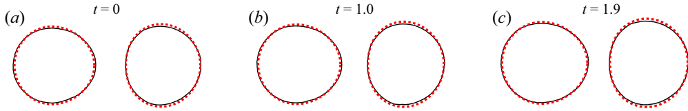
Figure 14. Experimental bubble shapes (black solid), asymptotic solution (6.5) and (6.8) (red dashed) for R = 1 , \delta = 2.86 and \sigma = (a) 2.68 , (b) 2.56 , (c) 2.43 . The corresponding dimensionless times t = \hat{t}\hat{U}/\hat{R}_1 are shown above for the experiments. The background flow is from left to right. Experimental images have been rescaled by the rear bubble radius, \hat{R}_1 = 5.4 mm, for comparison with the theory. The bubble shapes from experiment and asymptotics are aligned so that the centroids of the bubble pairs coincide.
