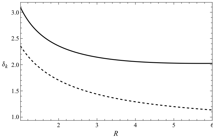
Figure 10. Minimum values \delta_1(R) (dashed) and \delta_2(R) (solid) of the Bretherton parameter, \delta , satisfying conditions i (see § 5.2.2) and ii (see § 5.2.3), respectively.
