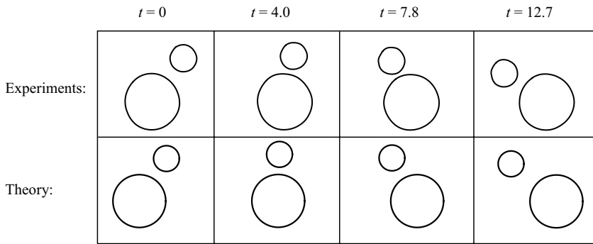
Figure 4. Two-bubble rollover with \delta = 1.17 and R = 2.05 at different dimensionless times t = \hat{t}\hat{U}/\hat{R}_1 . (top) Experimental images are compared with (bottom) simulations of the dimensionless dynamical system (3.17) with the same initial conditions at t = 0 . The background flow is from left to right. Experimental images have been rescaled by the rear bubble radius, \hat{R}_1 = 2.6 mm, for comparison with the theory.
