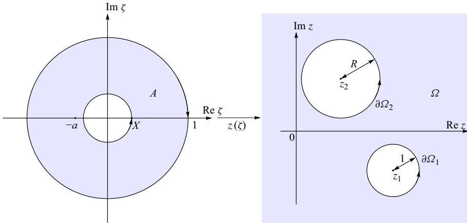
Figure 2. Schematic of the conformal map (3.1) from the annulus A = \{\zeta : X \leq |\zeta| \leq 1\} in the \zeta -plane to the fluid region \Omega in the z -plane.
