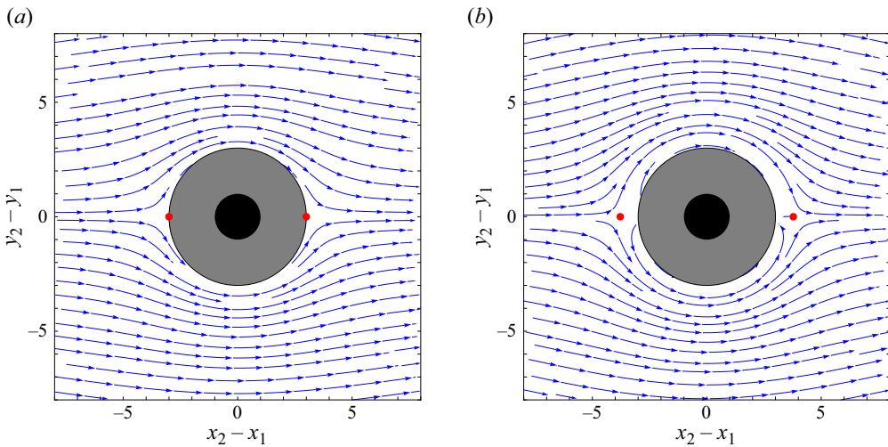
Figure 11. Trajectories for the two-bubble dynamical system (3.17) in the frame of the smaller bubble, with R=2 and (a) \delta=\delta_1(2) , at which the stationary points (shown as red points) lie on the surface |z_2 - z_1| = 1 + R , (b) \delta=\delta_2(2) , above which the separatrix encloses the region |z_2 - z_1| < 1 + R (solid grey fill). The solid black region |z_2 - z_1| \leq 1 represents the smaller bubble.
