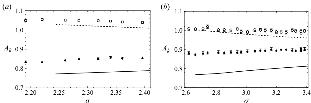
Figure 17. The bubble aspect ratios, A_k , versus separation, \sigma , for the rear bubble ( k = 1 , dashed curve and open markers) and the front bubble ( k = 2 , solid curve and filled markers), with (a) R = 1.23 , \delta = 2.55 and \epsilon = 0.03 (b), R = 1.65 , \delta = 1.94 and \epsilon = 0.05 . The points show experimental measurements, and the curves are the asymptotic predictions (6.10). The error between experiment and theory is approximately (a) 5 %–7 % and (b) 10 %–13 %.
