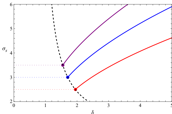
Figure 9. Position of the stationary point, \sigma_s , as a function of the Bretherton parameter, \delta , for radius ratios R = 1.5 (red), 2 (blue), 2.5 (purple). The dashed black curve shows where \sigma_s = 1 + R .
