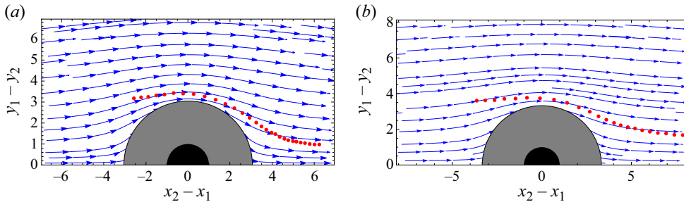
Figure 7. Trajectories for the two-bubble dynamical system (3.17) in the reference frame of the smaller bubble, with (a) \delta = 1.17 and R = 2.05 , (b) \delta = 0.90 and R = 2.32 . The blue vectors show the predicted trajectories of the centre of the larger bubble relative to the smaller one, and the red points show the experimentally measured bubble positions. Error bars are comparable to the size of the markers and are thus omitted. Any trajectories entering the solid grey region |z_2 - z_1| \leq (1 + R) are such that the two bubbles will collide. The solid black region |z_2 - z_1| \leq 1 represents the smaller bubble.
