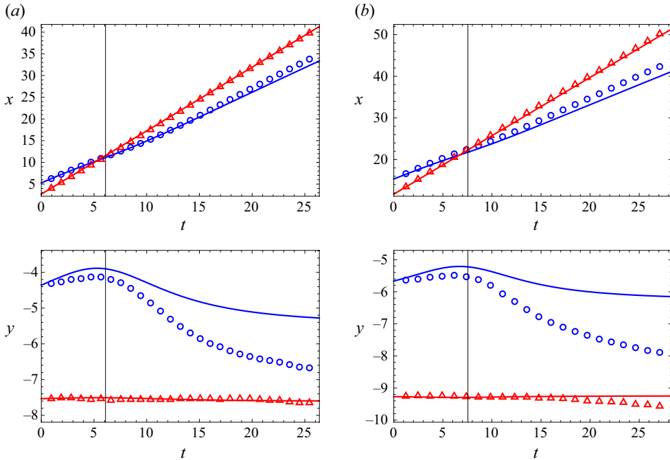
Figure 6. The positions of the bubble centres (x, y) (top and bottom, respectively) versus dimensionless time t for (a) \delta = 1.17 and R = 2.05 , (b) \delta = 0.90 and R = 2.32 . Solid lines show theoretical predictions, and points show experimental data. The bubble of unit radius ( k = 1 ) is shown in blue (circles), and the bubble of radius R ( k = 2 ) is shown in red (triangles). In each plot, the time at which x_1 = x_2 is shown with a vertical line. Error bars are comparable to the size of the markers and are thus omitted.
