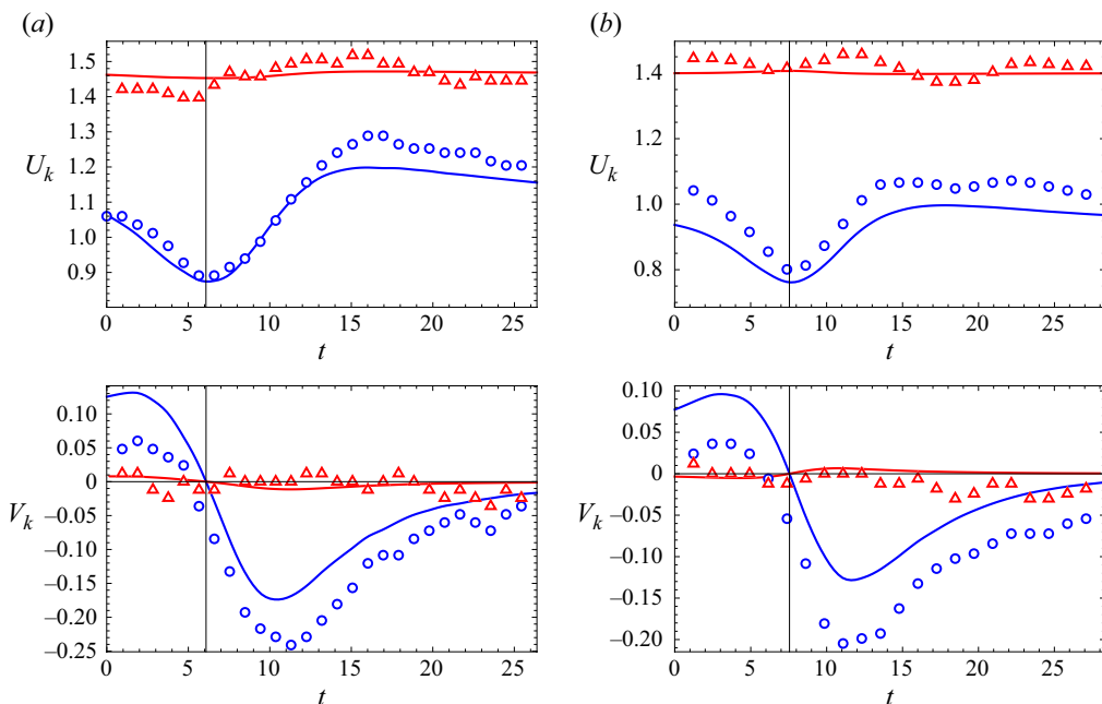
Figure 5. The instantaneous bubble velocity components ( U_k , V_k ) (top and bottom, respectively) versus dimensionless time t for (a) \delta = 1.17 and R = 2.05 , (b) \delta = 0.90 and R = 2.32 . Solid lines show theoretical predictions and points show experimental data. The bubble of unit dimensionless radius ( k = 1 ) is shown in blue (circles), and the bubble of radius R ( k = 2 ) is shown in red (triangles). In each plot, the time at which x_1 = x_2 is shown with a vertical line. Error bars are comparable to the size of the markers and are thus omitted.
