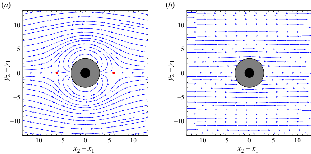
Figure 8. Trajectories for the two-bubble dynamical system (3.17) in the reference frame of the smaller bubble, with R = 2 and (a) \delta = 5 , (b) \delta = 1/2 . Any trajectories entering the solid grey region |z_2 - z_1| \leq (1 + R) are such that the two bubbles will collide. Stationary points are shown in red. The solid black region |z_2 - z_1| \leq 1 represents the smaller bubble.
