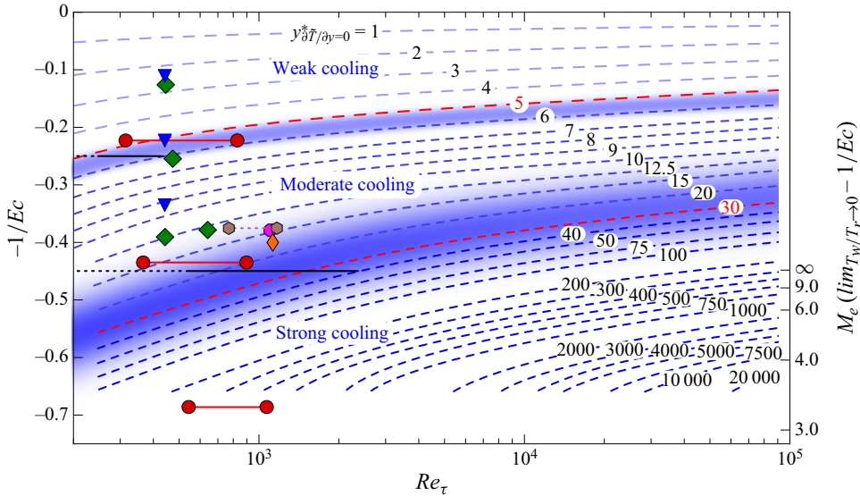
Figure 4. Regime diagram for the cooled cases as -1/Ec over Re_\tau . The dashed curved denote the estimated position of y_{\partial\tilde{T}/\partial y=0}^* and the proposed location of the regime change are marked as red curves. The symbols and lines denote the position where the reference data are located in the plot. The two black lines mark the location of the bounds plotted in figure 1 for the DNS data range 400 \lesssim Re_\tau \lesssim 1200 . The right axis marks the Mach number M_e at the equivalent -1/Ec in the limit value \tilde{T}_w/\tilde{T}_r \rightarrow 0 .
