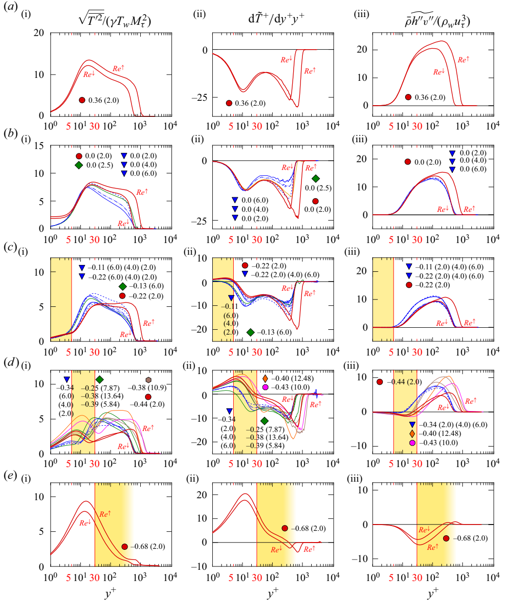
Figure 8. Plot of the inner-scaled temperature fluctuation (labelled as (i) in the left column), the pre-multiplied temperature gradient (labelled as (ii) in the middle column) and the normalized turbulent heat flux (labelled as (iii) in the right column). The rows, from top to bottom, correspond to the regimes: (a) heated, (b) adiabatic, (c) weakly cooled, (d) moderately cooled and (e) strongly cooled. Each data point is identified by its respective value of -1/Ec and Mach number in brackets ( M_e ). The legend in figure 1 includes the references for the line colours and symbols.
