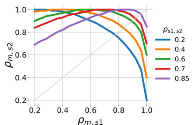
Figure 1 (Srivastava et al.). All points below the x = y line on each of the curves indicate a situation where model m is guaranteed to perform worse in predicting s2 data when fitted to s1 data.
