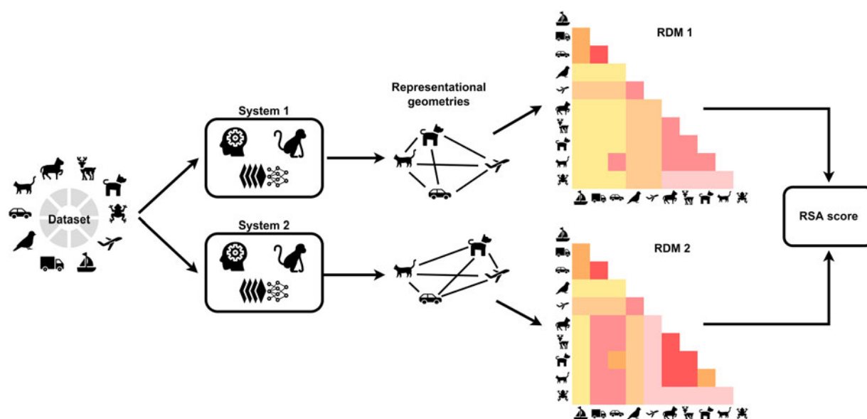
Figure 3. RSA calculation. A series of stimuli from a set of categories (or conditions) are used as inputs to two different systems (e.g., a brain and a DNN). The corresponding neural or unit activity for each stimulus is recorded and pairwise distances in the activations within each system are calculated to get the representational geometry of each system. This representational geometry is expressed as a representational dissimilarity matrix (RDM) for each system. Finally, an RSA score is determined by computing the correlation between the two RDMs (image taken from Dujmović et al., 2022).
